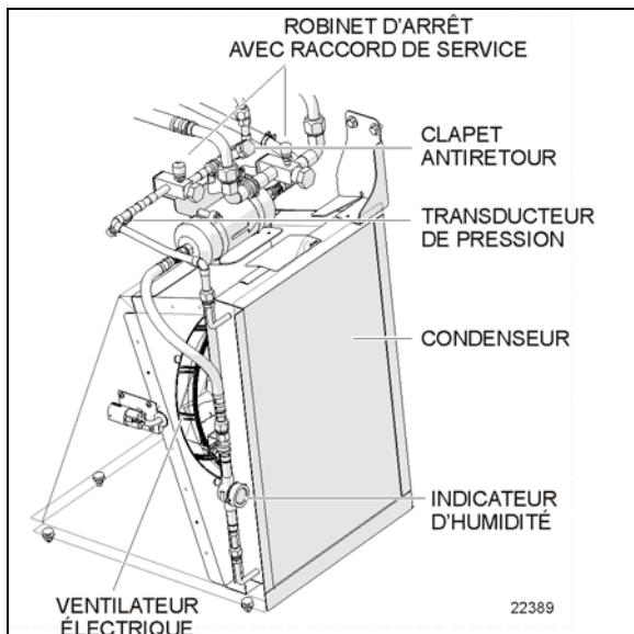
FIGURE 86: CONFIGURATION DE CONDENSEUR X3-45 VIP
