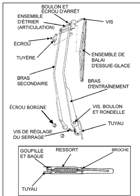
FIGURE 36: ESSUIE-GLACE INFÉRIEUR
