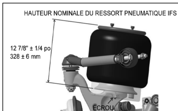
FIGURE 33: RESSORTS PNEUMATIQUES
