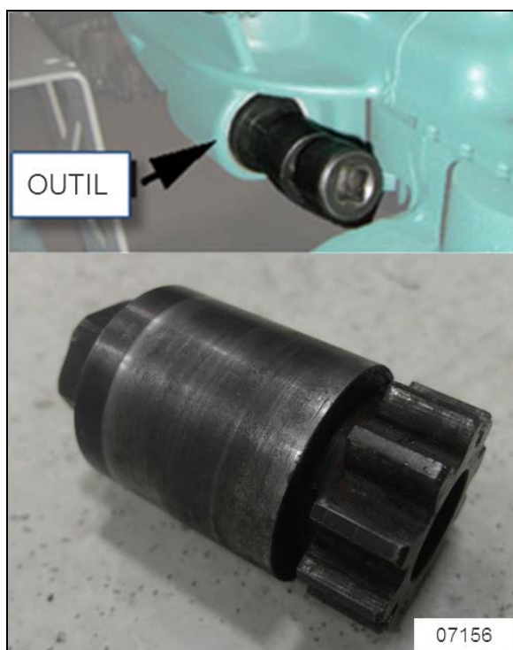
FIGURE 10: OUTIL VOLVO #88800014
