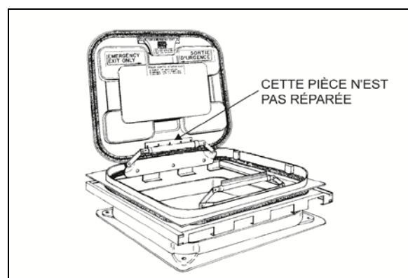
FIGURE 23: TRAPPE D'ÉVACUATION 18104
