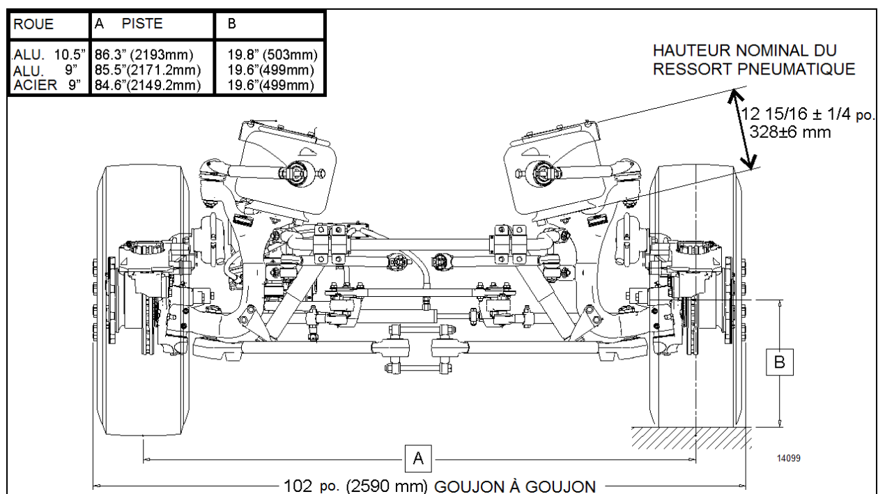
FIGURE 36: DIMENSIONS NOMINALES IFS
