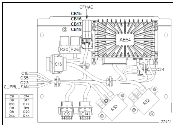
FIGURE 64: MODULE CVAC
