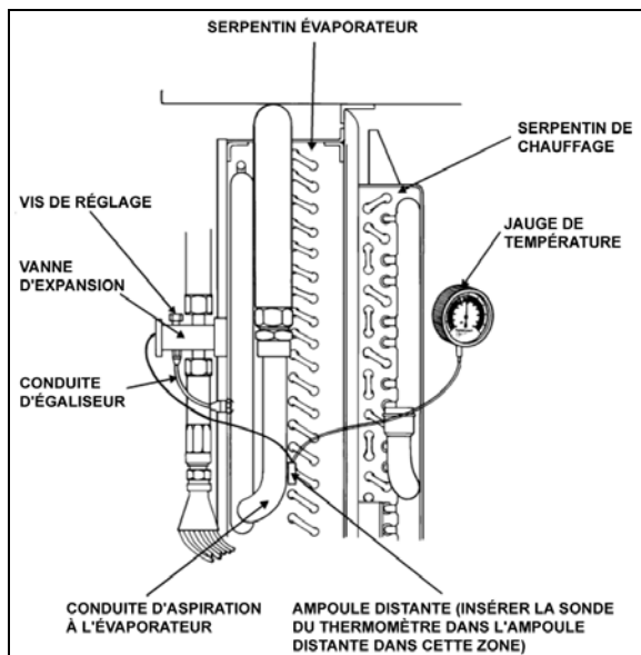
FIGURE 57: AJUSTEMENT DE LA SURCHAUFFE. INSTALLATION
