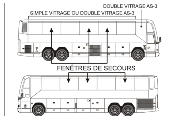
FIGURE 30: AUTOCAR H3-41 18520
