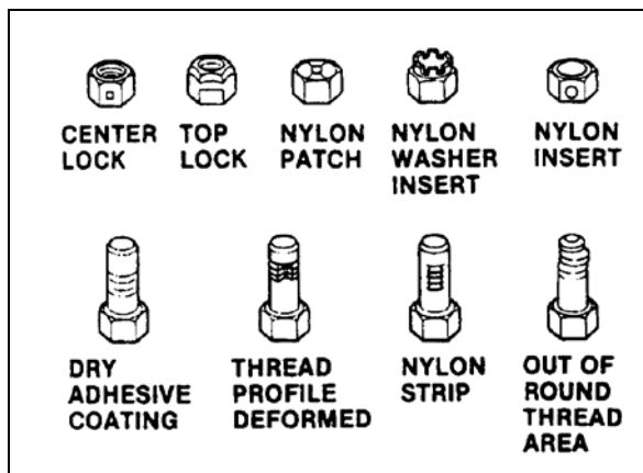
FIGURE 13: ATTACHES AUTOBLOQUANTES
