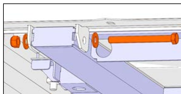
FIGURE 23: BOULON TRANSVERSAL, 2 EMBLEMENTS
