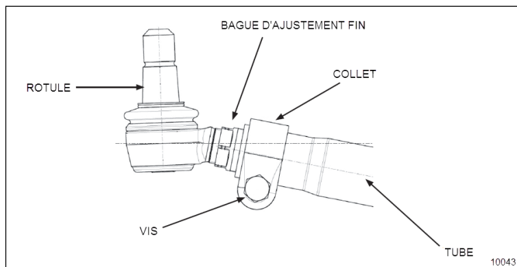
FIGURE 2: COMPOSANTES DE LA BIELLE
