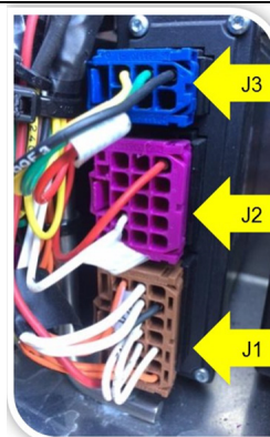
FIGURE 11: MODULE I/O-EA
