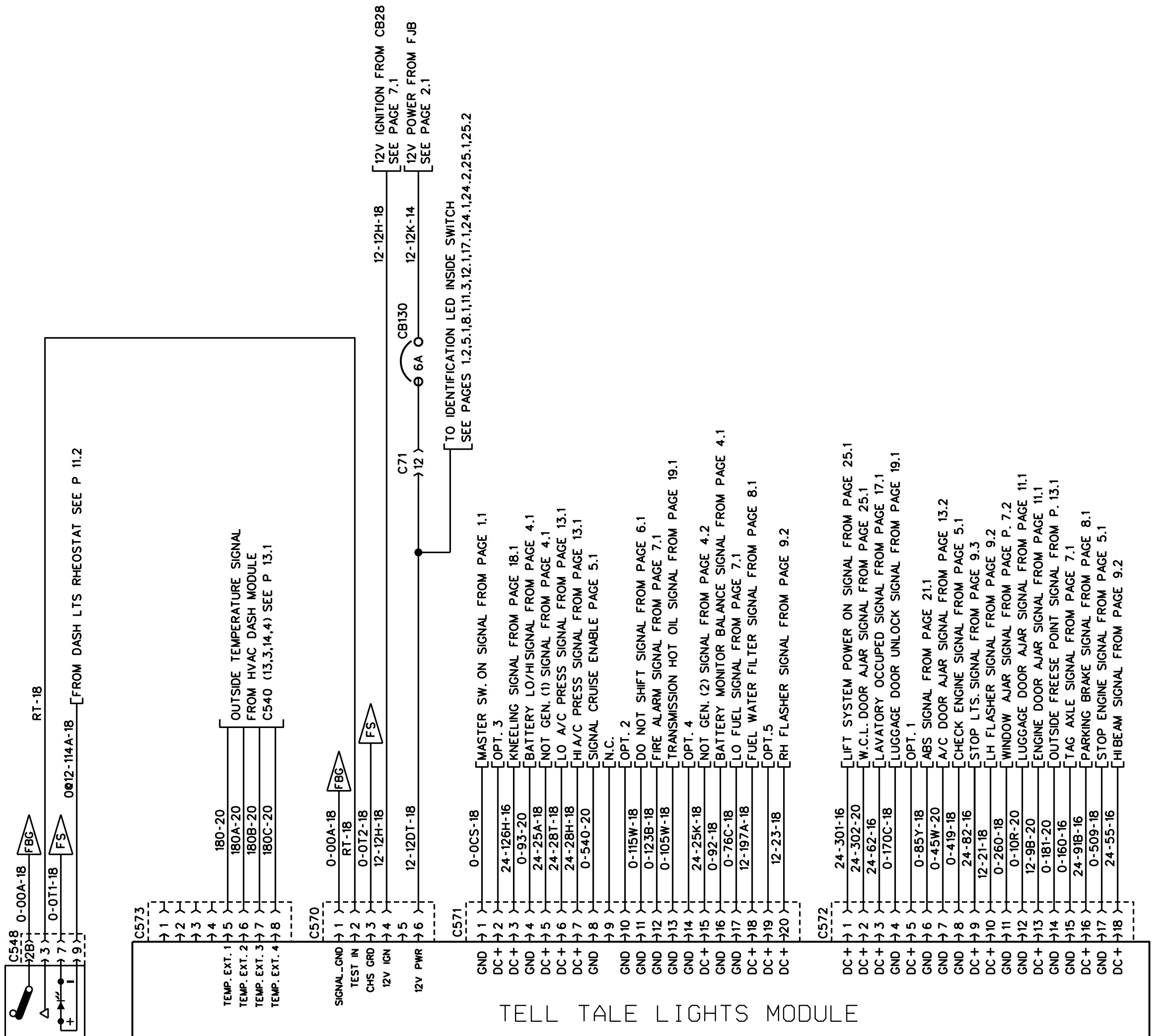
TELL TALE LIGHT MODULES
