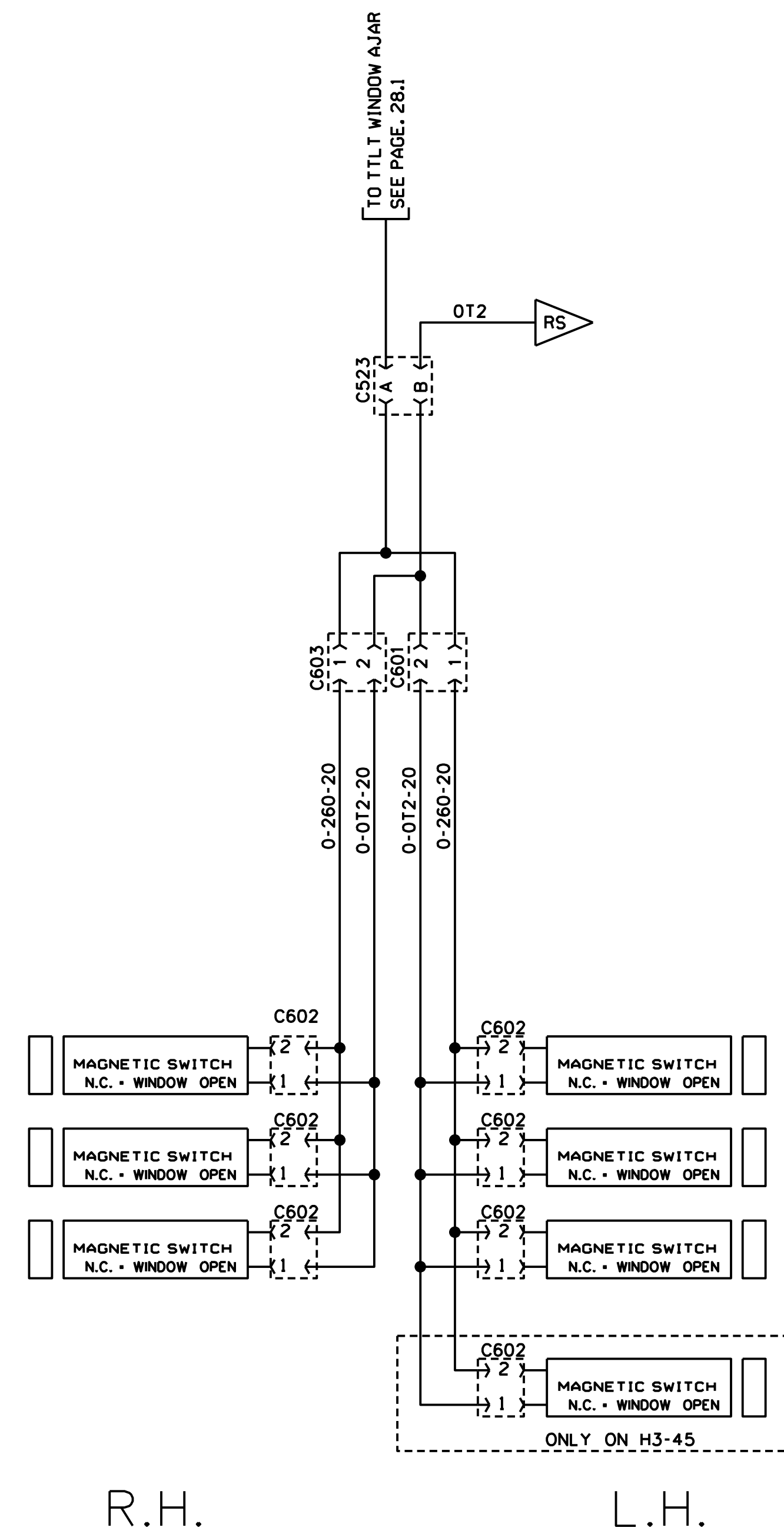
WINDOW AJAR
