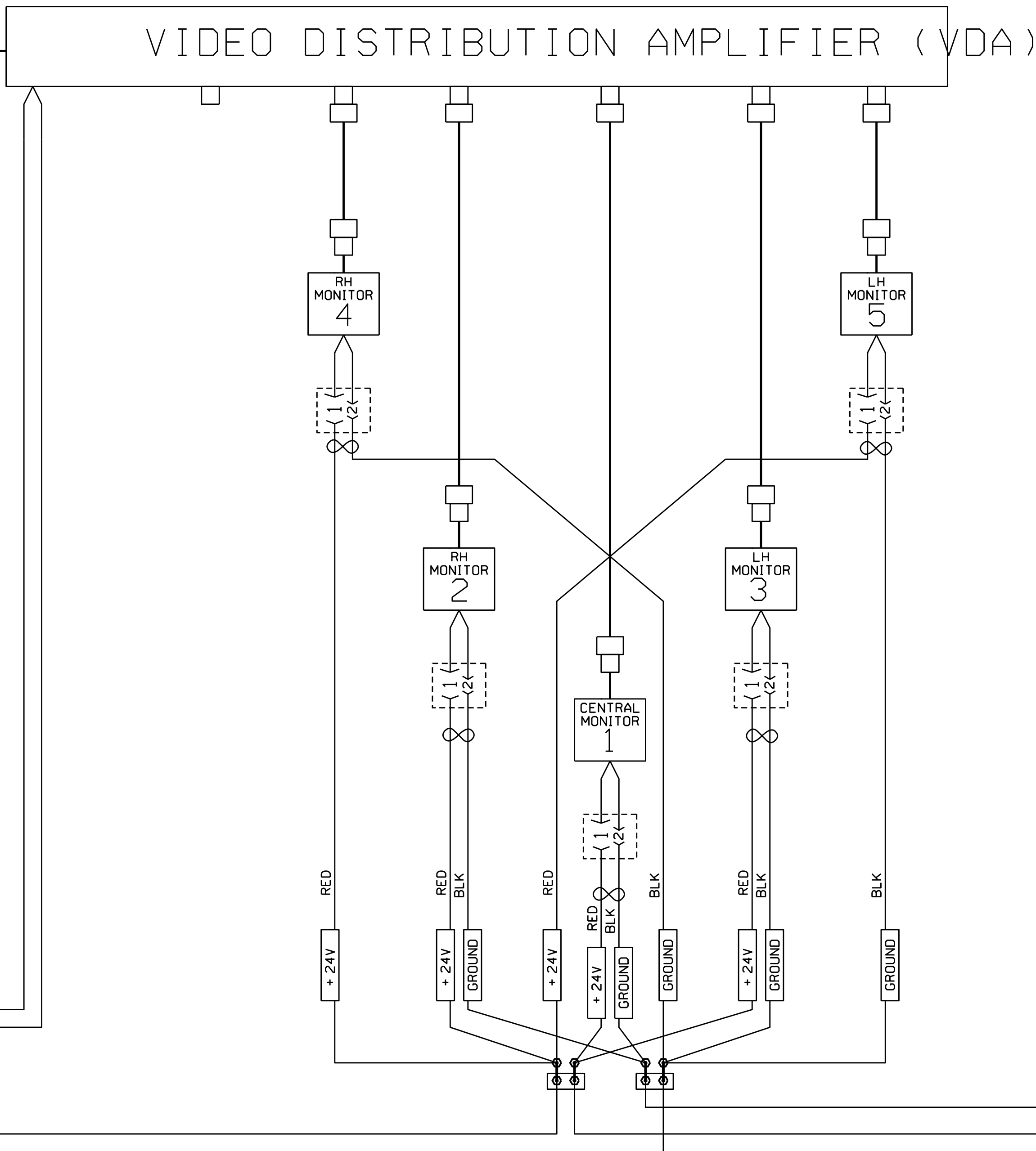
VIDEO SYSTEM
