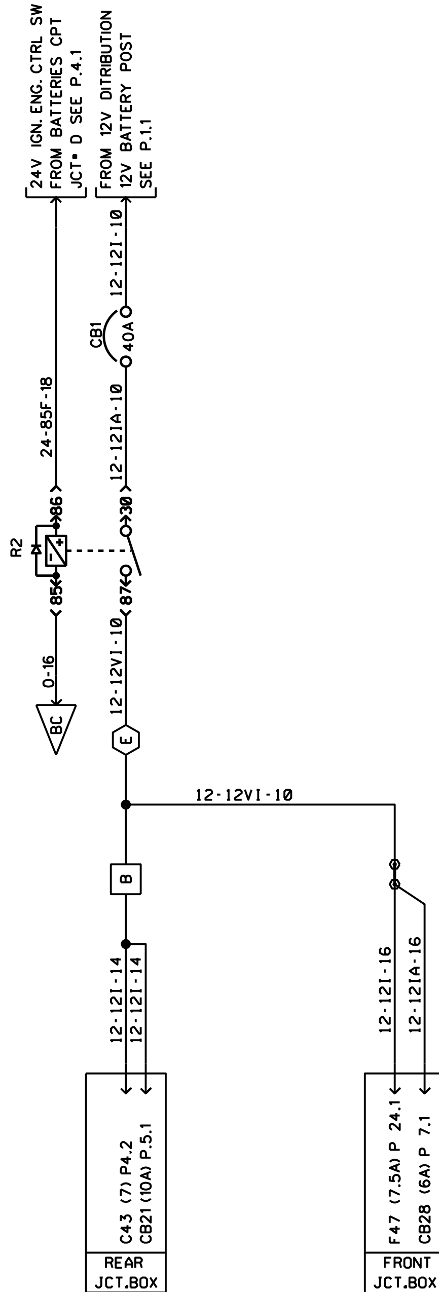
12V IGNITION
