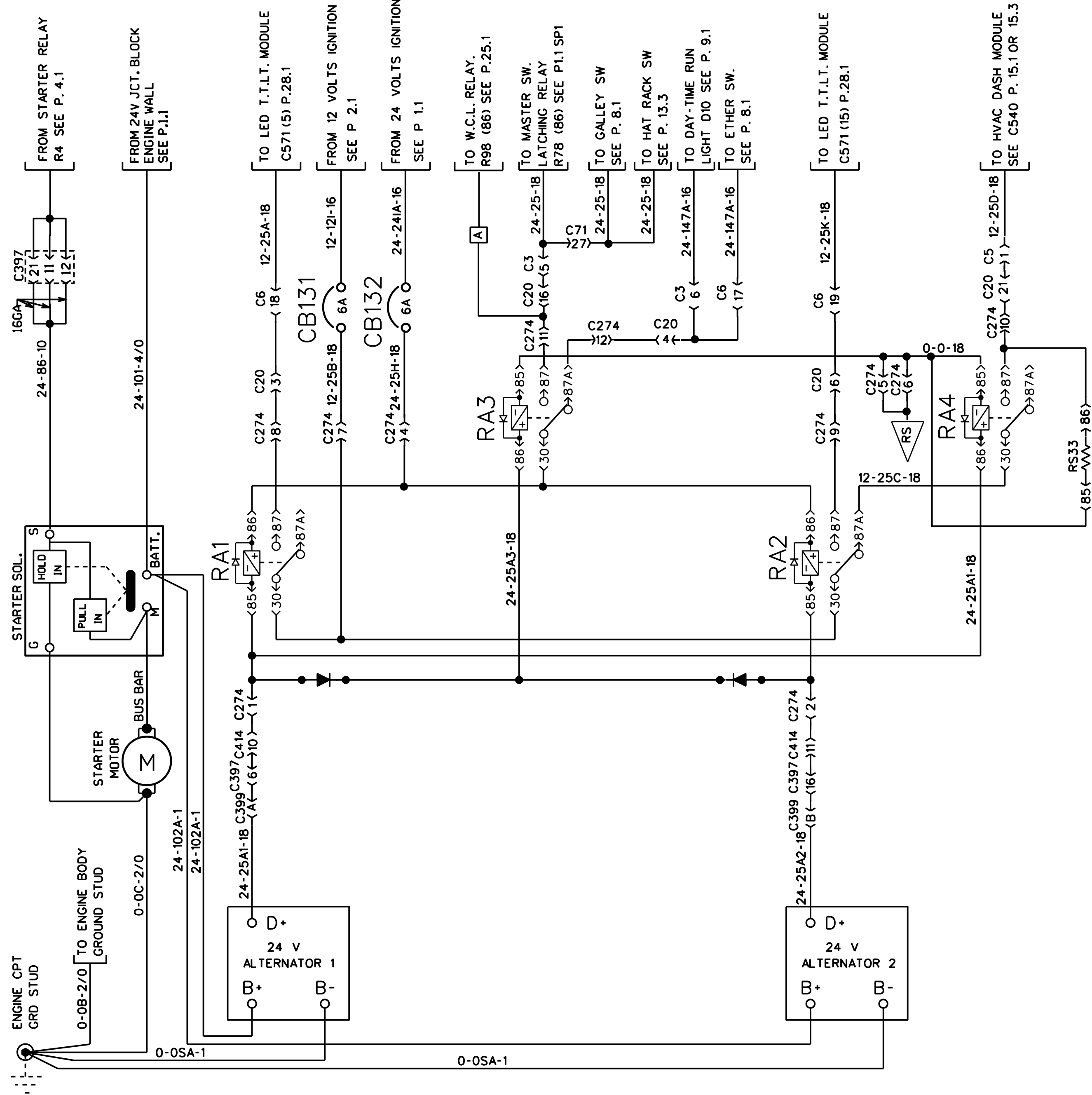
STARTER & ALTERNATOR BOSCH
