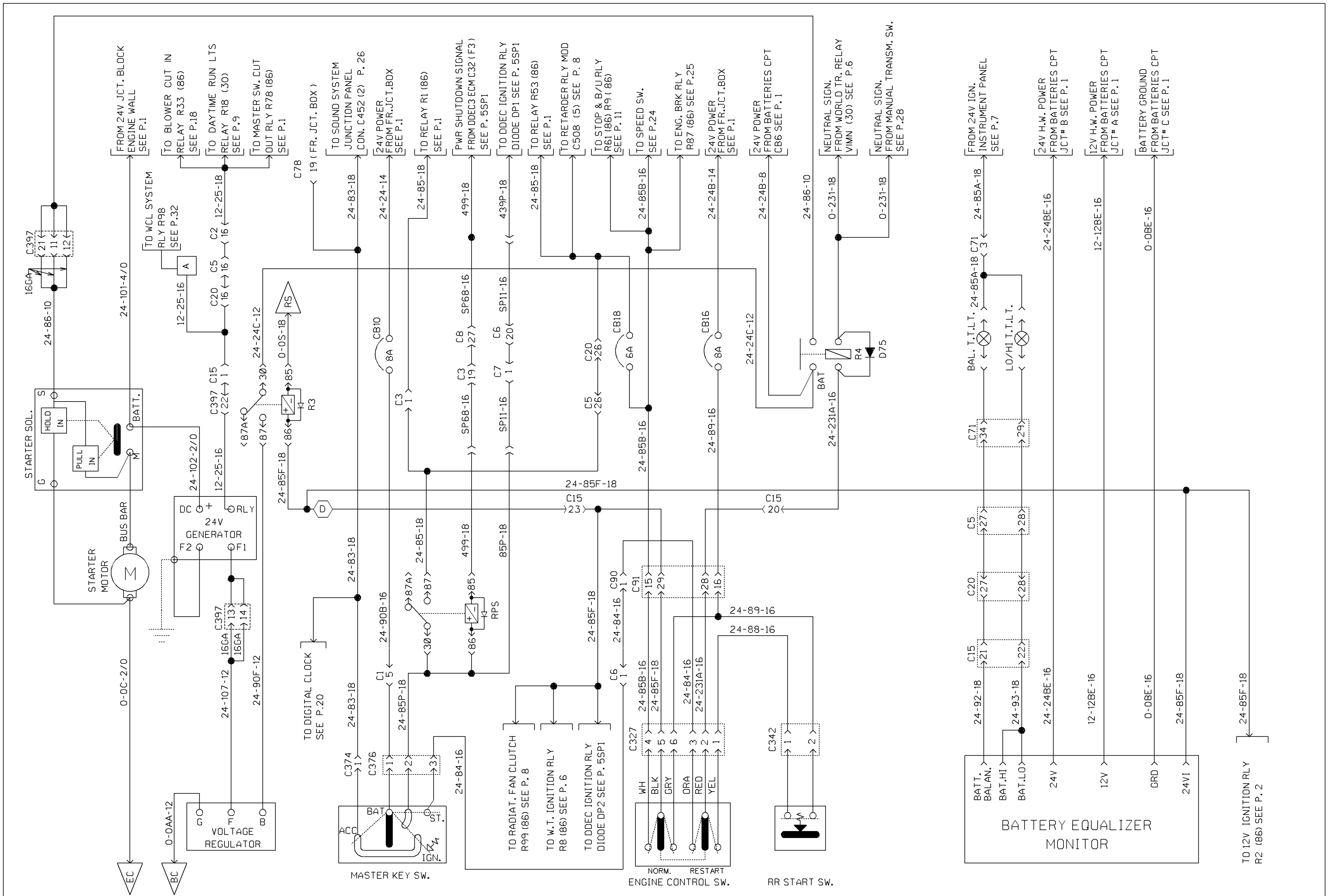
SPECIAL CHARGING SYSTEM & ENGINE CONTROL WITH POWER SHUTDOWN & IDLE TIMER
