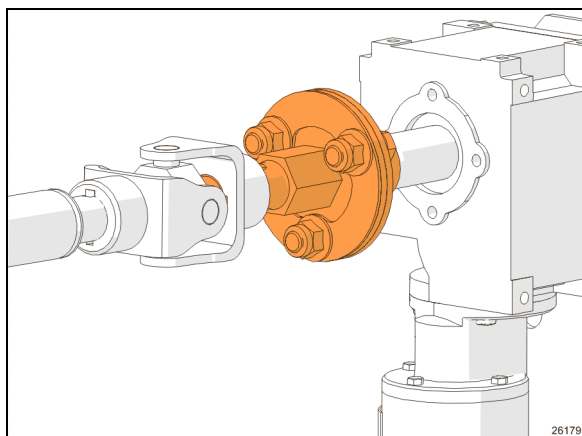
FIGURE 37: BRIDE AJUSTABLE
