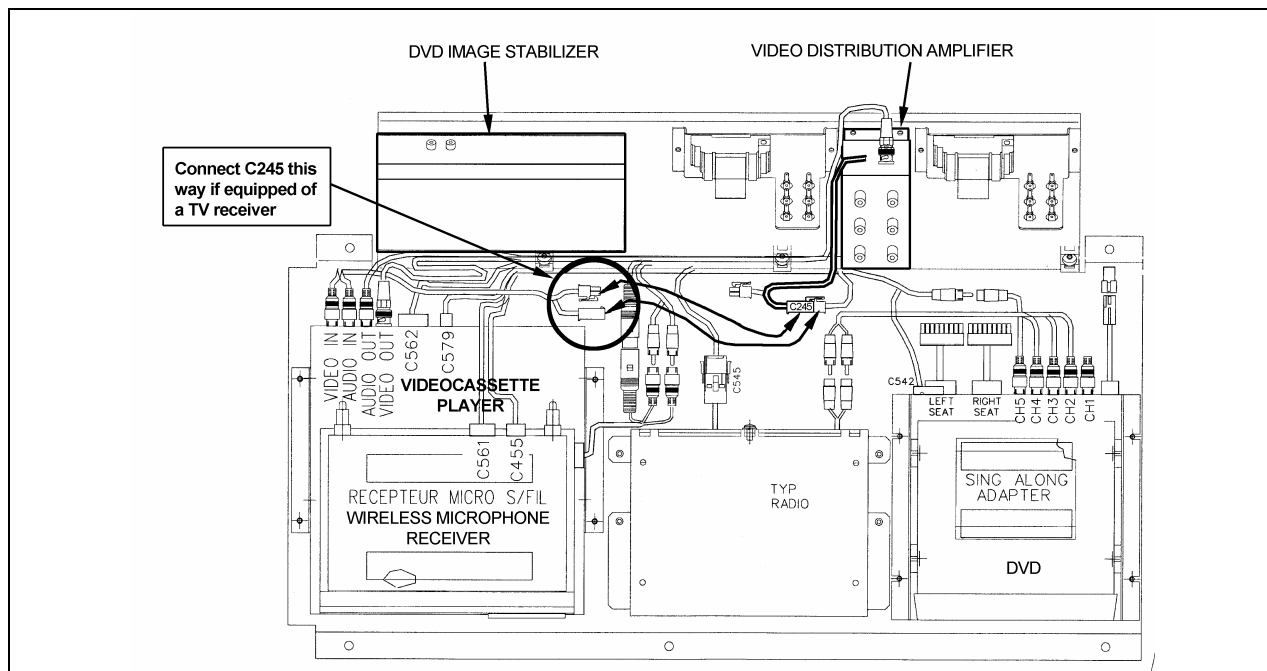
FIGURE 1: AUDIO/VIDEO ACCESSORY PANEL
