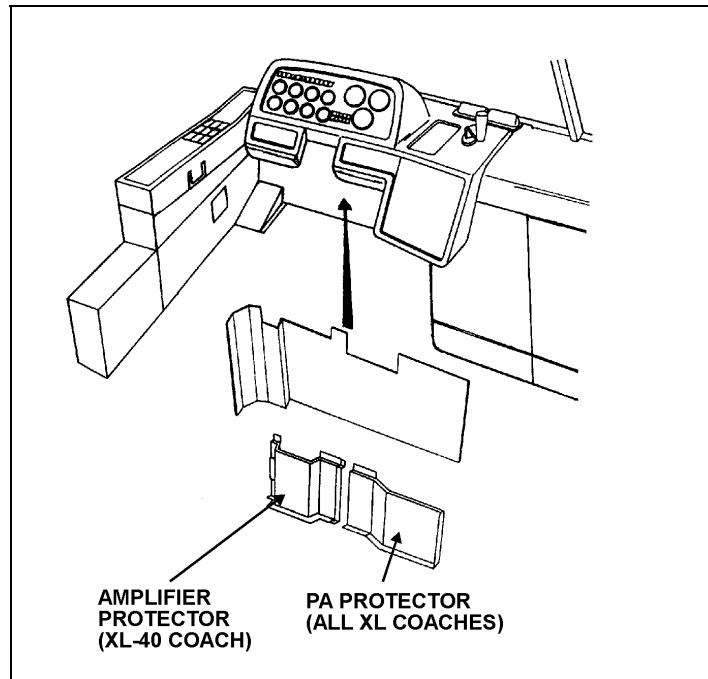
FIGURE 3: DASHBOARD - AMPLIFIER LOCATION ON XL-40 COACHES
