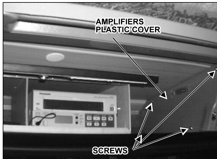
FIGURE 4: INSIDE FORWARD L.H. PARCEL RACK (BEHIND DRIVER) - AMPLIFIERS LOCATION ON XL-45 COACH
