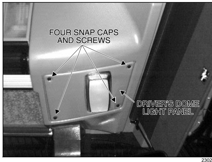
23029 FIGURE 2: - DOME LIGHT PANEL AMPLIFIER(S) LOCATION ON H3 COACHES
