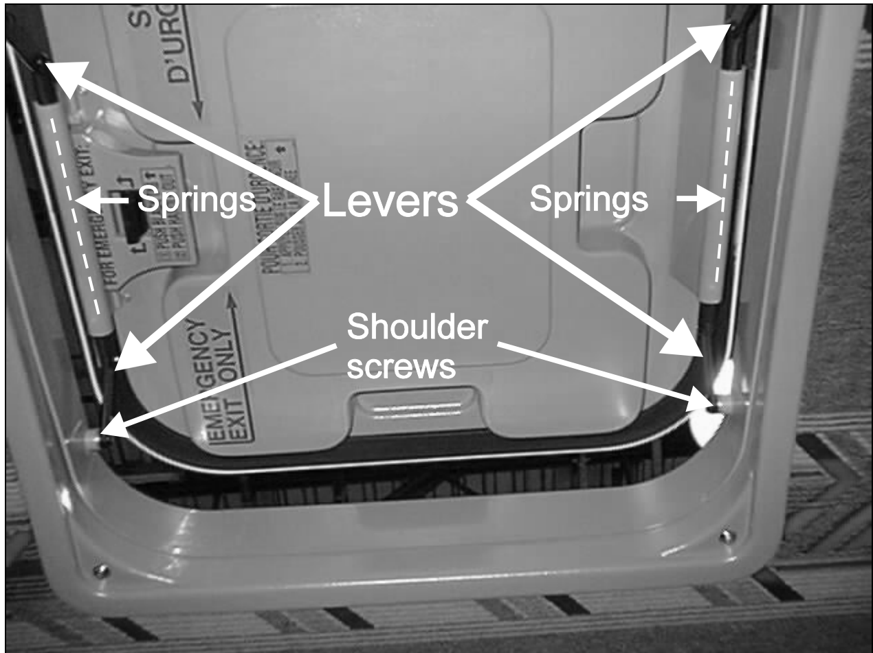
FIGURE 1: H3-45 ROOF VENTILATION HATCH
