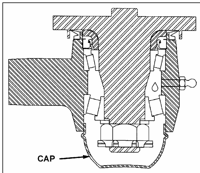
FIGURE 2: INSTALLATION OF NEW CAP
