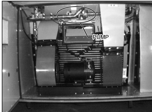
FIGURE 3: HVAC COMPARTMENT
