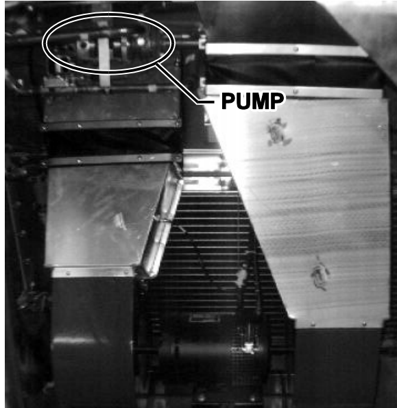
FIGURE 2: HVAC COMPARTMENT
