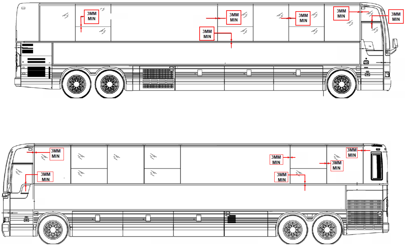
FIGURE 1 : 3MM (0.118in) MINIMUM GAP TO BE RESPECTED (X3 VIP SHOWN)
