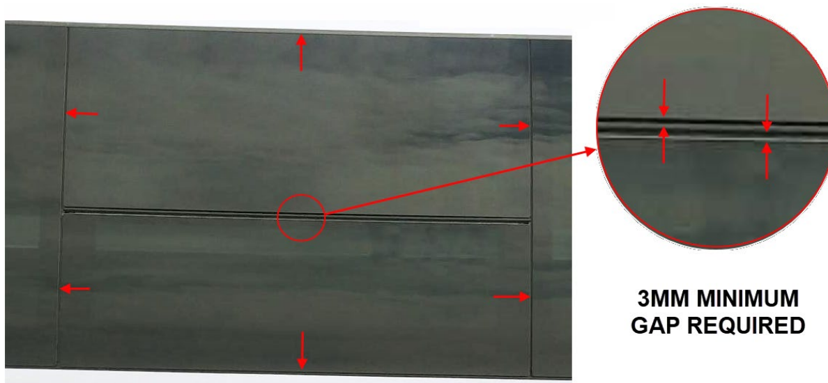
FIGURE 3 : SLIDE OUT 3MM GAP DETAILS
