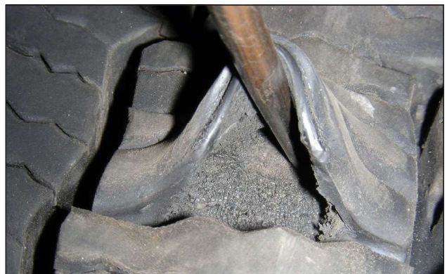
EFFECT: Internal Deterioration of the Tread Rubber CAUSE: Prolonged Use of Dynamometer
