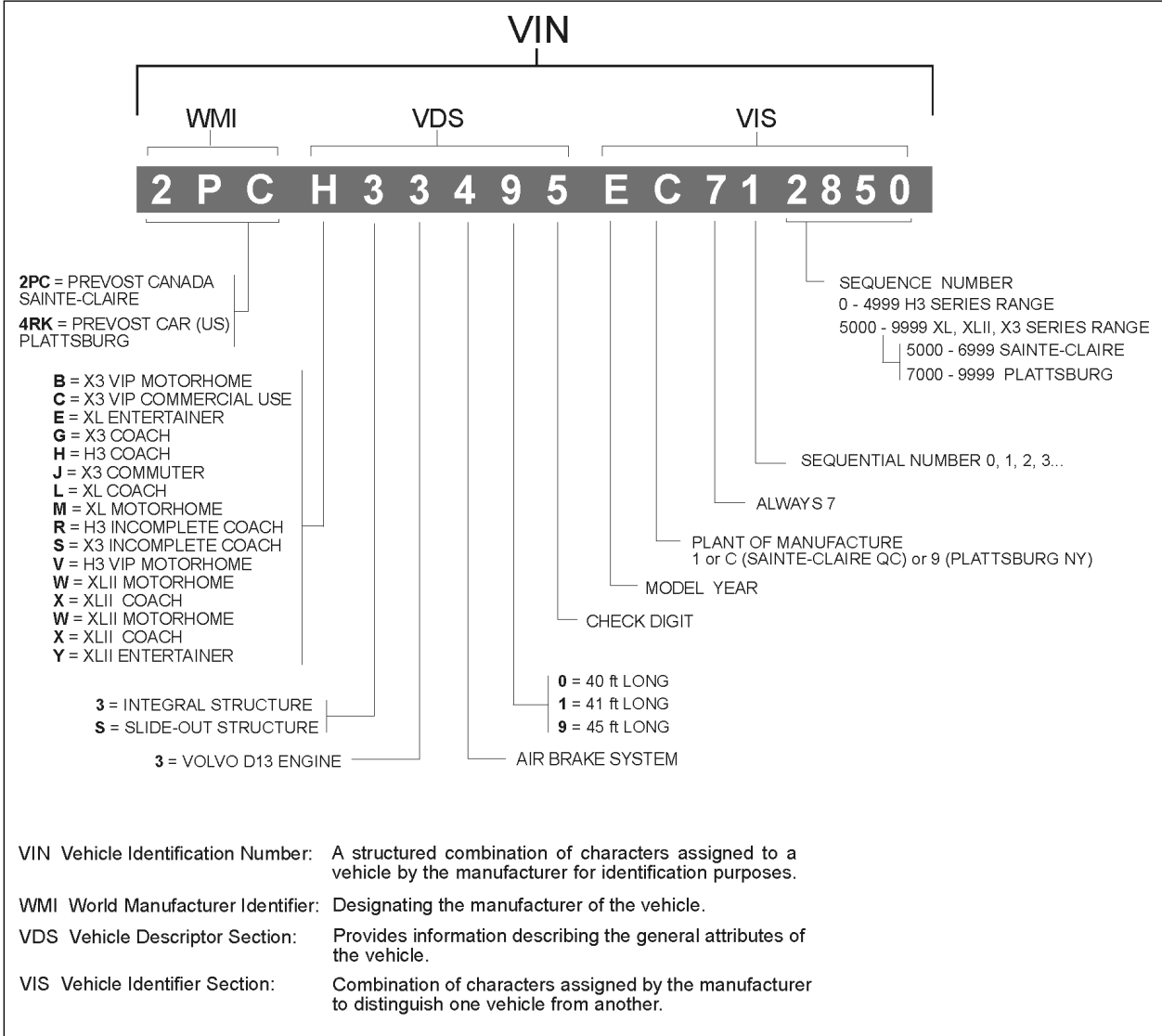
FIGURE 10: VEHICLE IDENTIFICATION NUMBER – UP TO 2024
