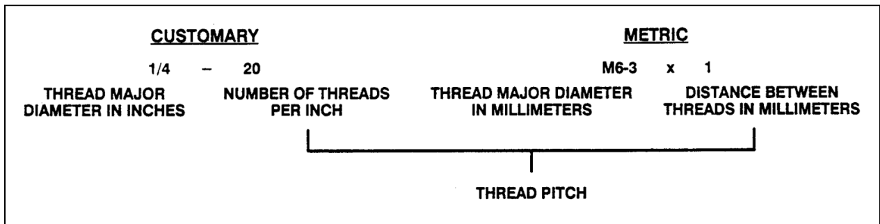
FIGURE 12: THREAD NOTATION
