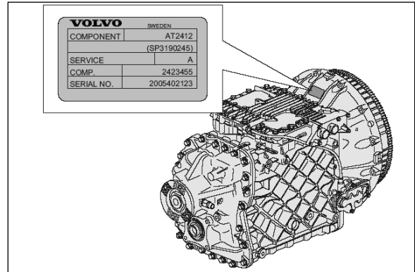
FIGURE 3: I-SHIFT TRANSMISSION
