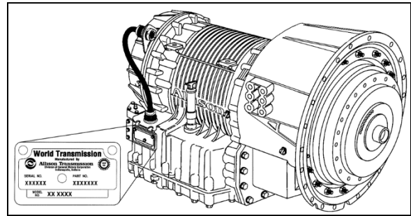
FIGURE 2: ALLISON TRANSMISSION 07076
