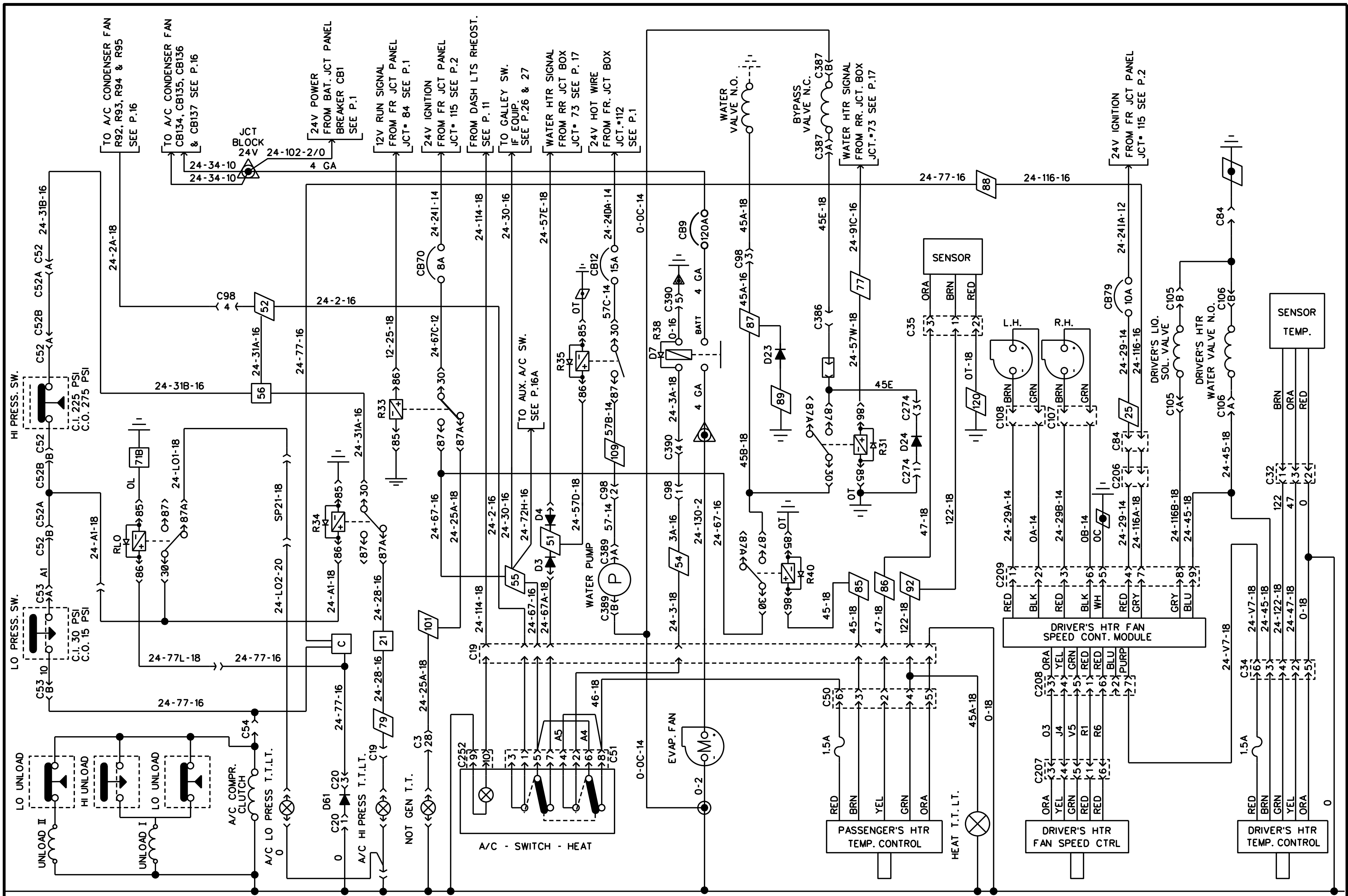
SPECIAL A/C AND HEAT SYSTEM WITH A/C HI - LO PRESS. T. T. LT.
