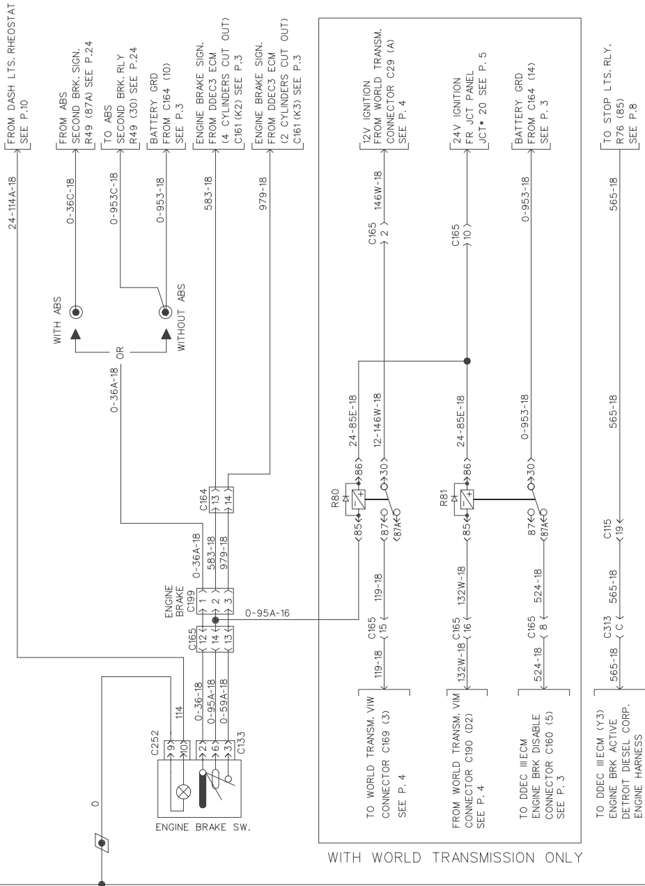
ENGINE BRAKE SYSTEM
