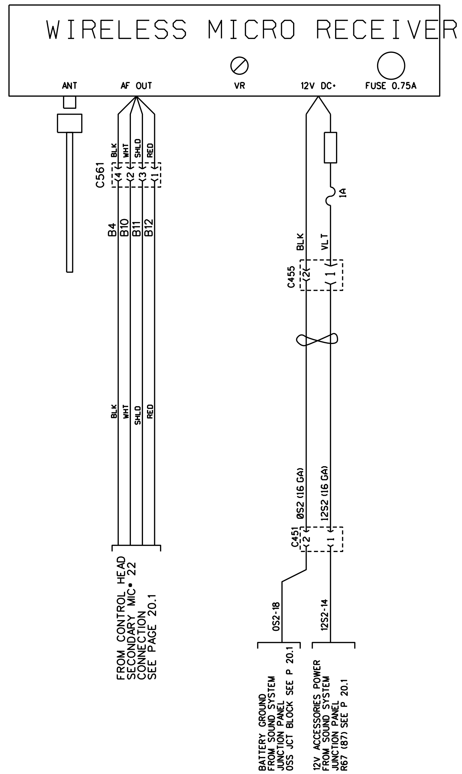
WIRELESS MICROPHONE
