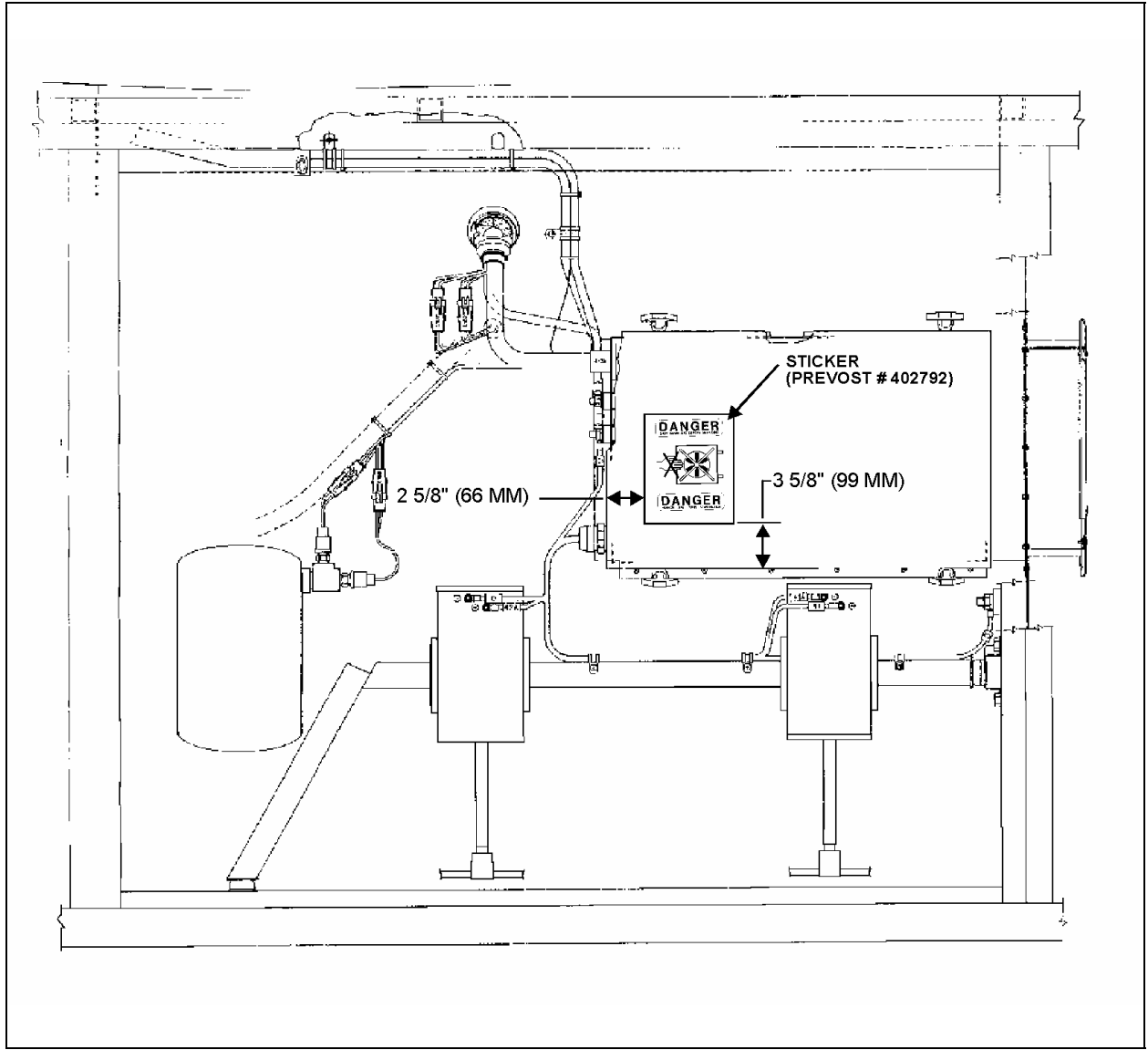
FIGURE 1: CONDENSER COMPARTMENT
