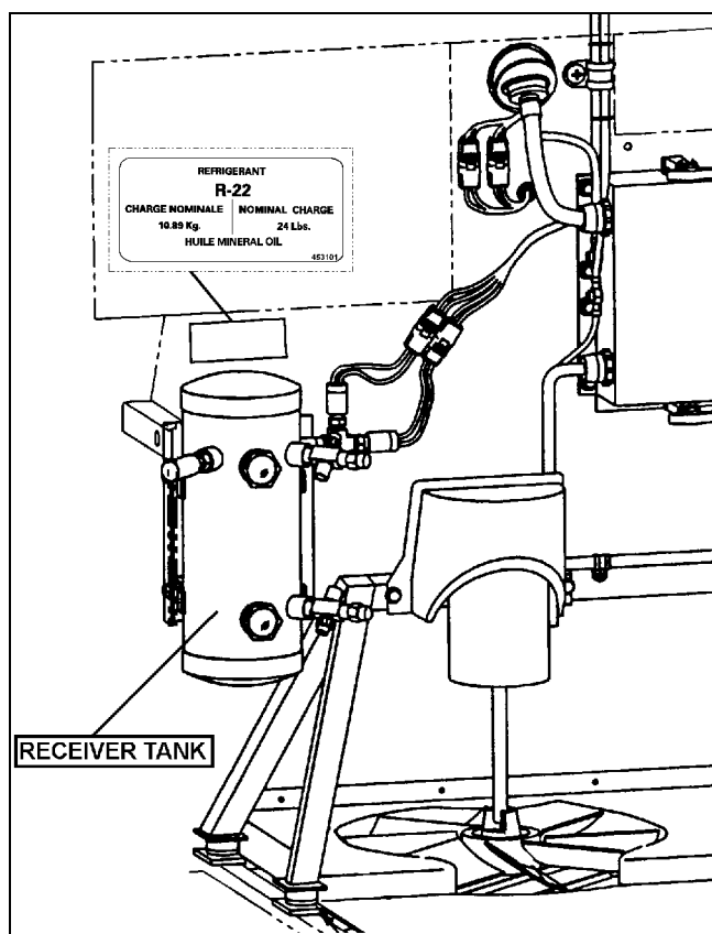
FIGURE 2: CONDENSER COMPARTMENT
