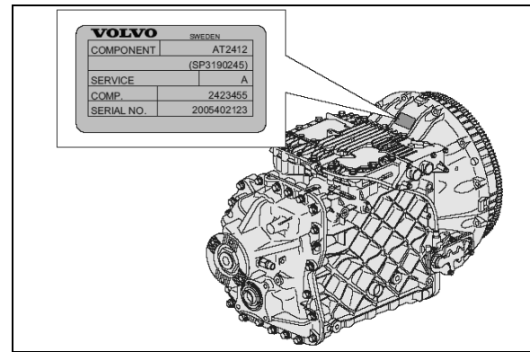
FIGURE 3: I-SHIFT TRANSMISSION
