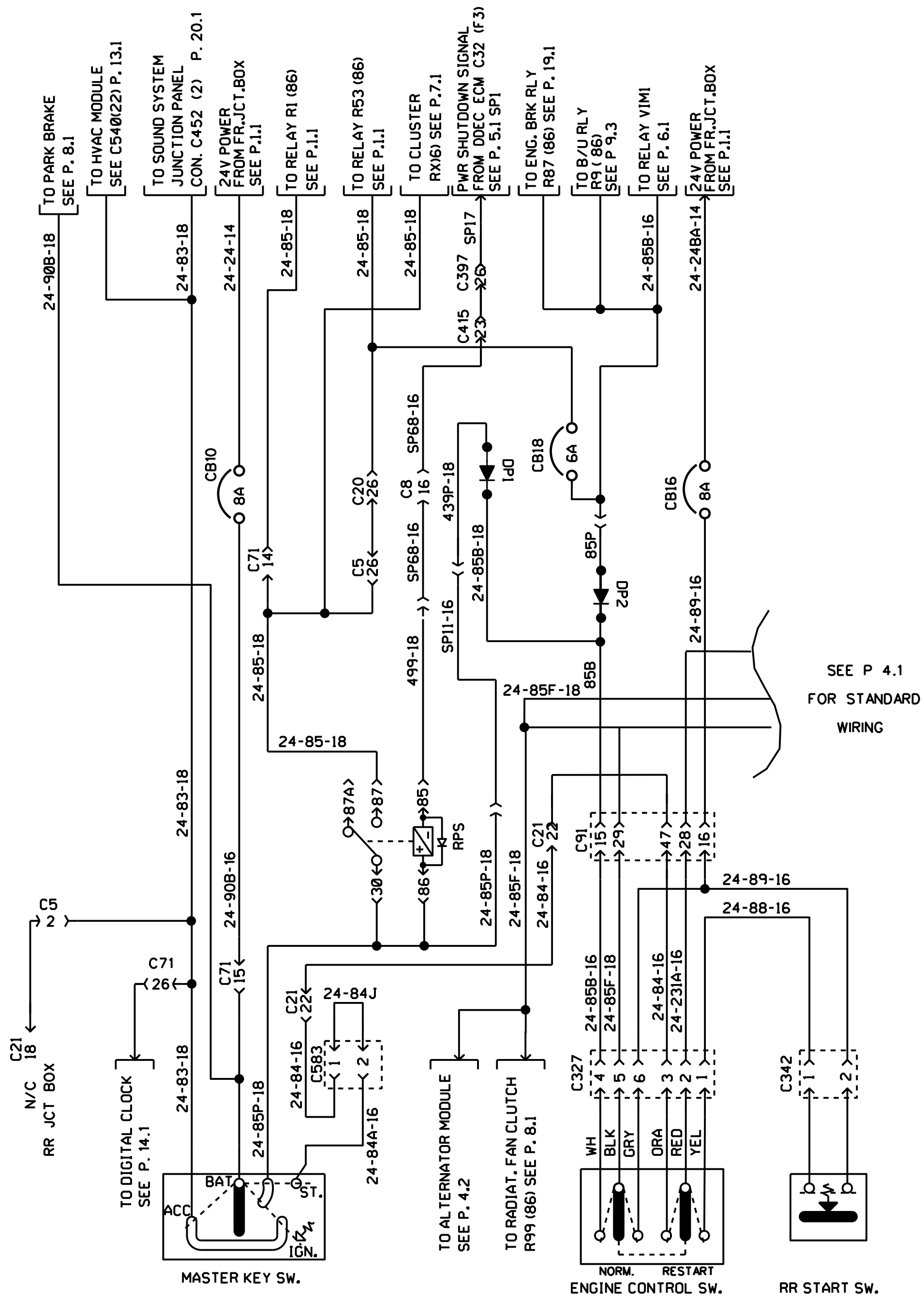
ENGINE CONTROL WITH POWER SHUTDOWN & IDLER TIMER
