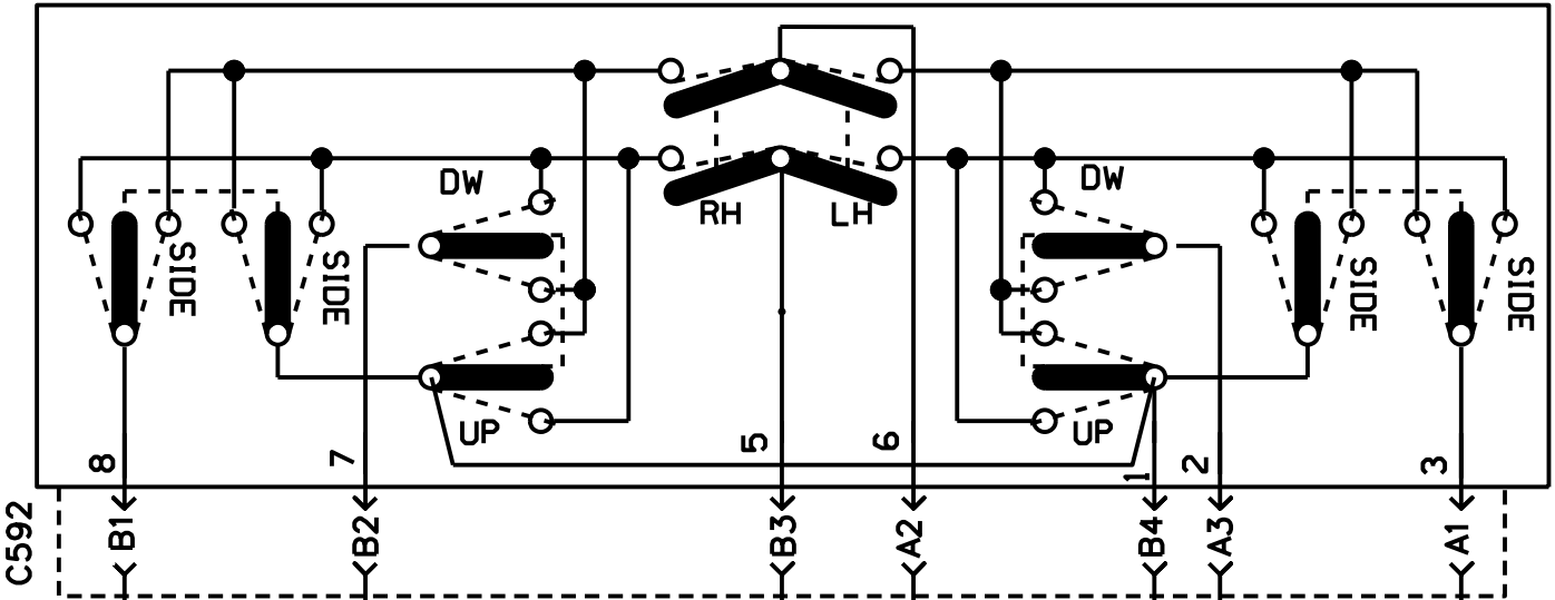
ADJUST FLAT & CONVEX RH MIRROR SWITCH
