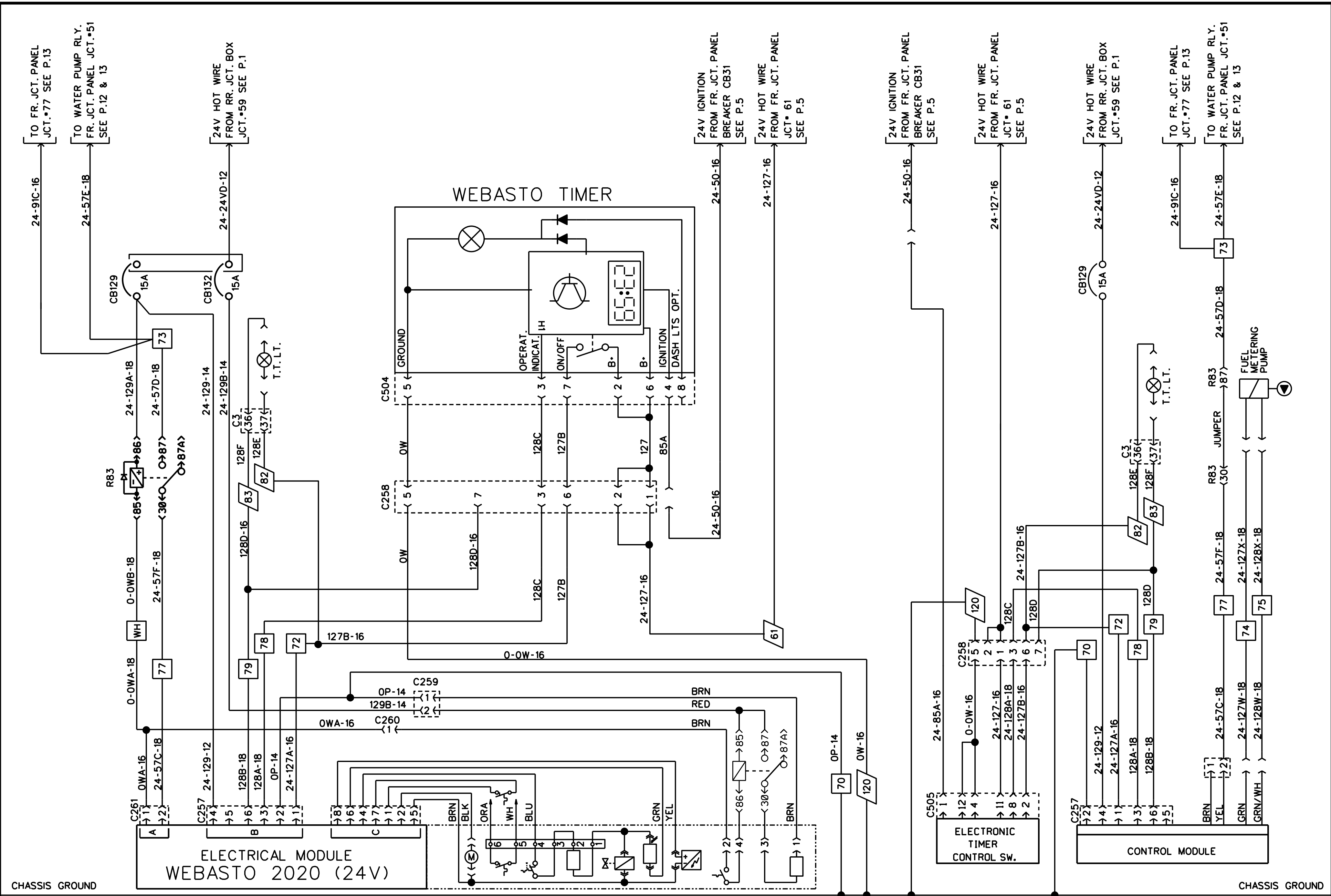
PRE-HEAT WATER HEATER WEBASTO 2020
