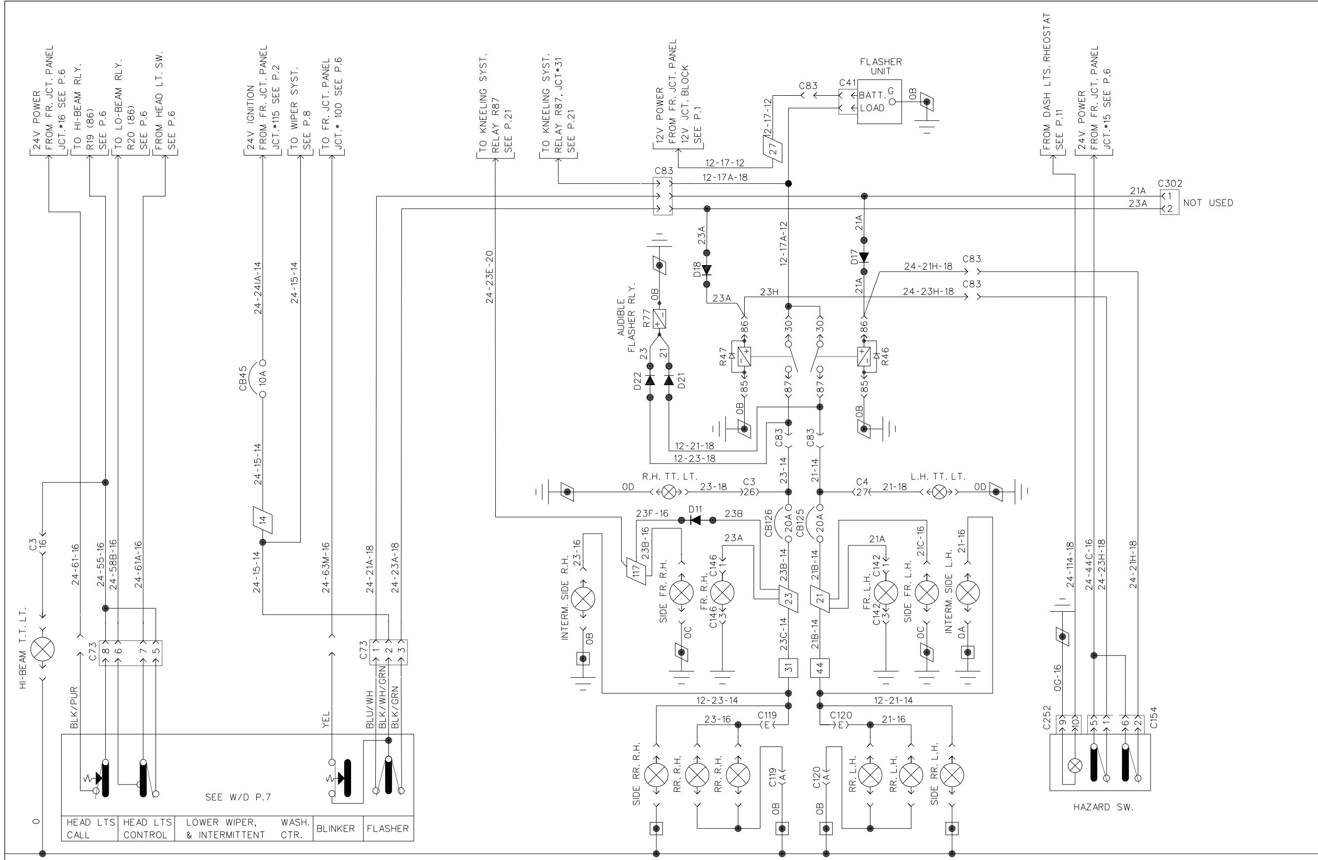
CHASSIS GROUND MULTI-FUNCTION LEVEL CTR. SW. DIRECTIONAL AND HAZARD LTS. CHASSIS GROUND
