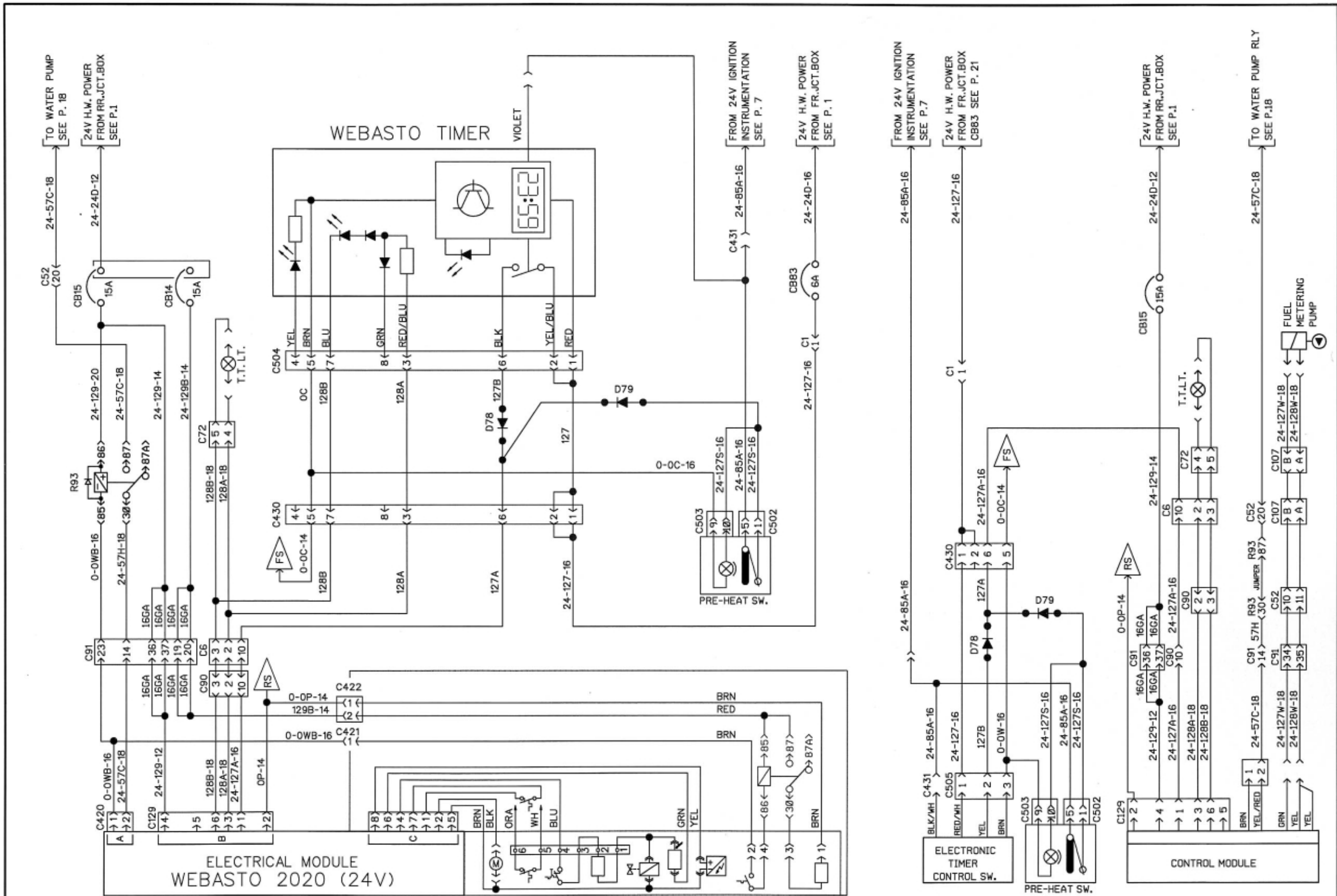
PRE-HEAT WATER HEATER (WEBASTO 2020)
