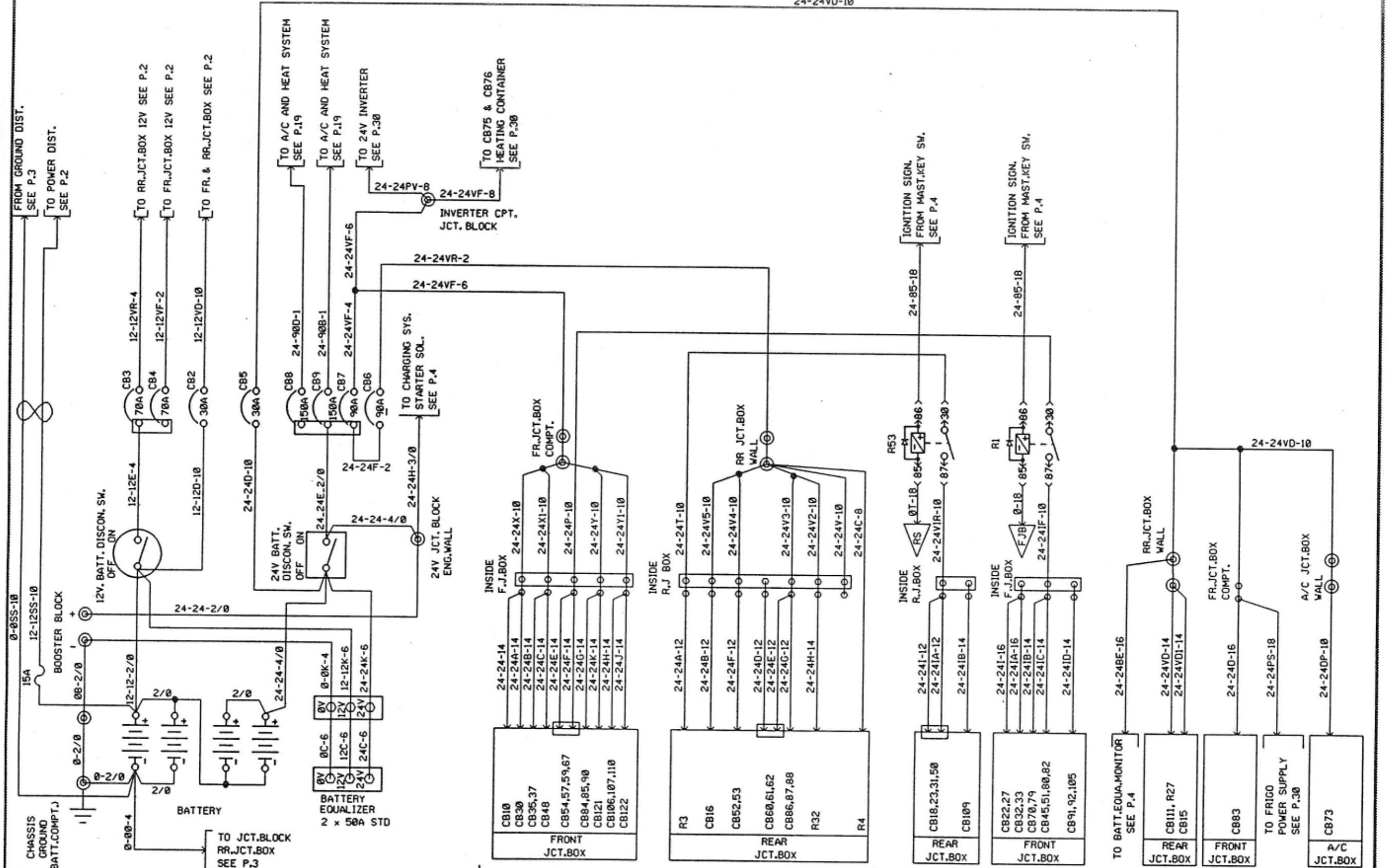
12V,24V DISTRIBUTION
