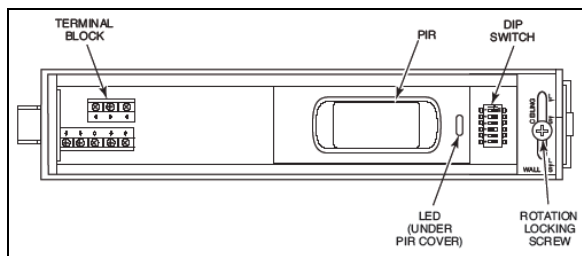
FIGURE 25: LAVATORY LIGHT MOTION SENSOR
