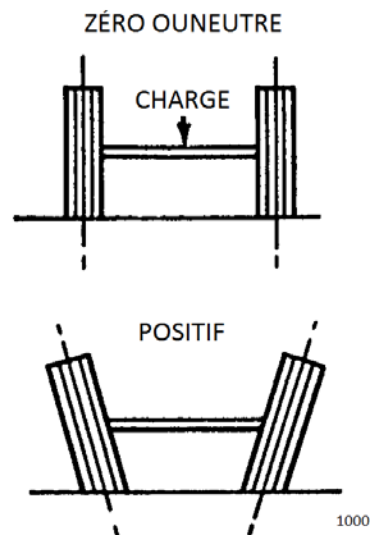
FIGURE 3: ANGLE DE CARROSSAGE
