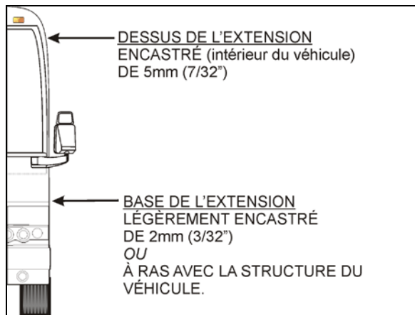
FIGURE 27: AJUSTEMENT 26055
