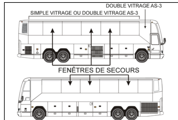
FIGURE 30: AUTOCAR H3-41 18520
