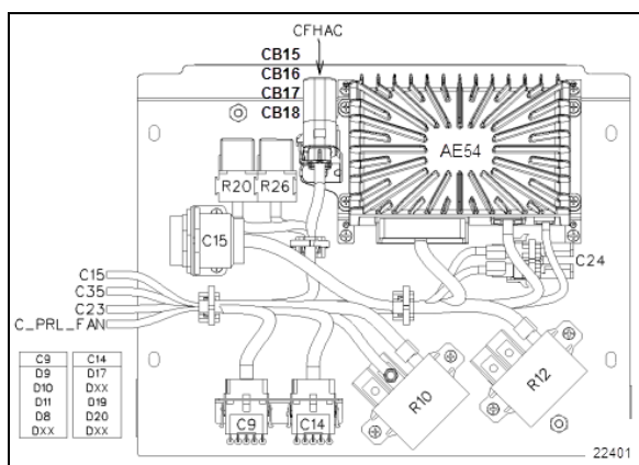
FIGURE 62: MODULE CVC
