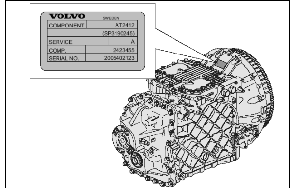
FIGURE 3: TRANSMISSION I-SHIFT
