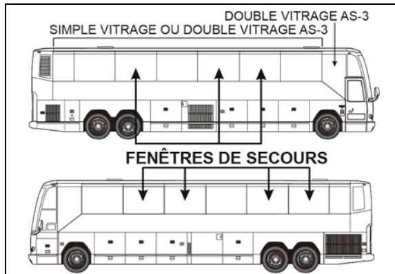
FIGURE 29: AUTOCAR H3-45 18519
