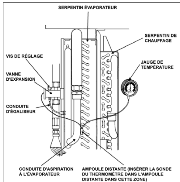
FIGURE 55: AJUSTEMENT DE LA SURCHAUFFE. INSTALLATION
