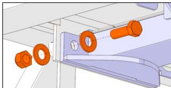
FIGURE 24: BOULON LONGITUDINAL, 4 EMBLEMENTS
