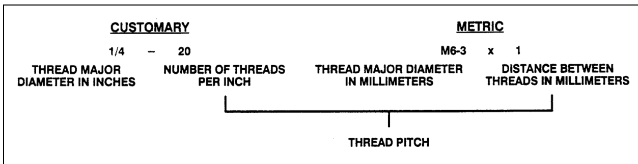
FIGURE 12: THREAD NOTATION
