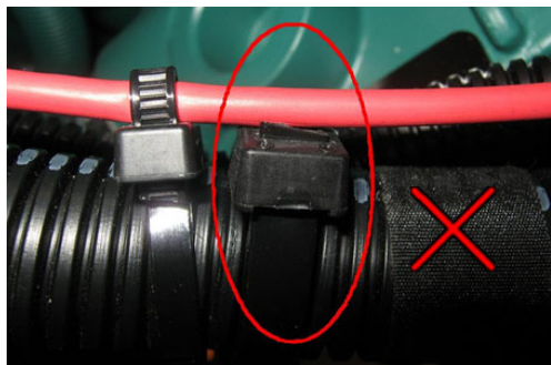
LTD touching cut cable tie
