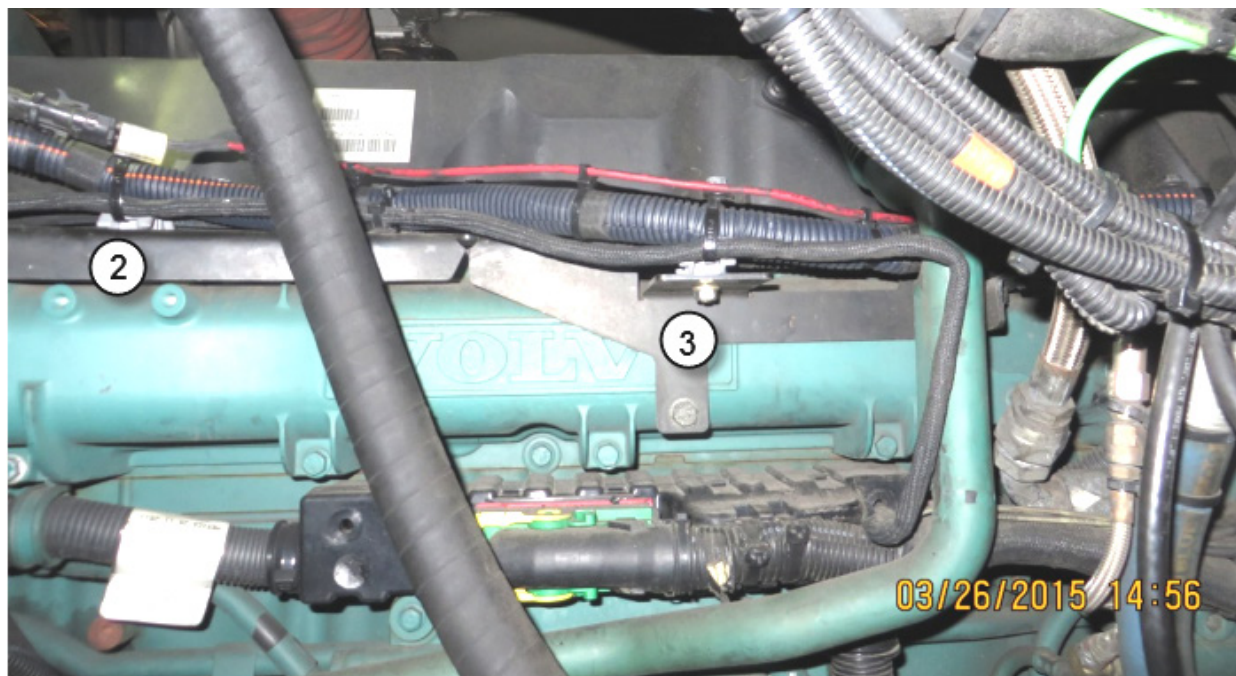
FIGURE 16: POWER CABLE ATTACHED TO #2, #3 DOUBLE-TIE MOUNT AND PROPER NYLON TIES INSTALLATION
