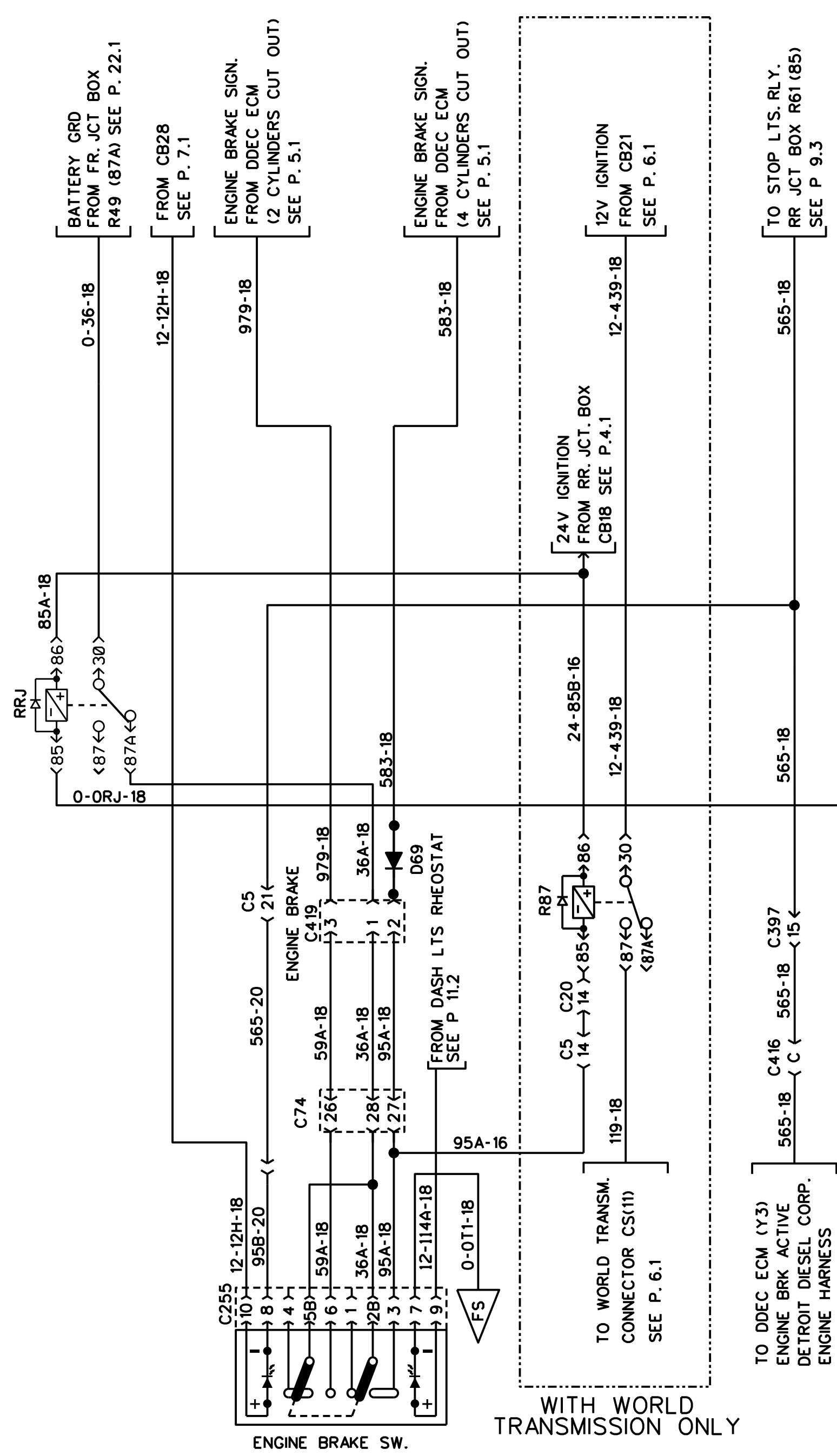
ENGINE BRAKE SYSTEM
