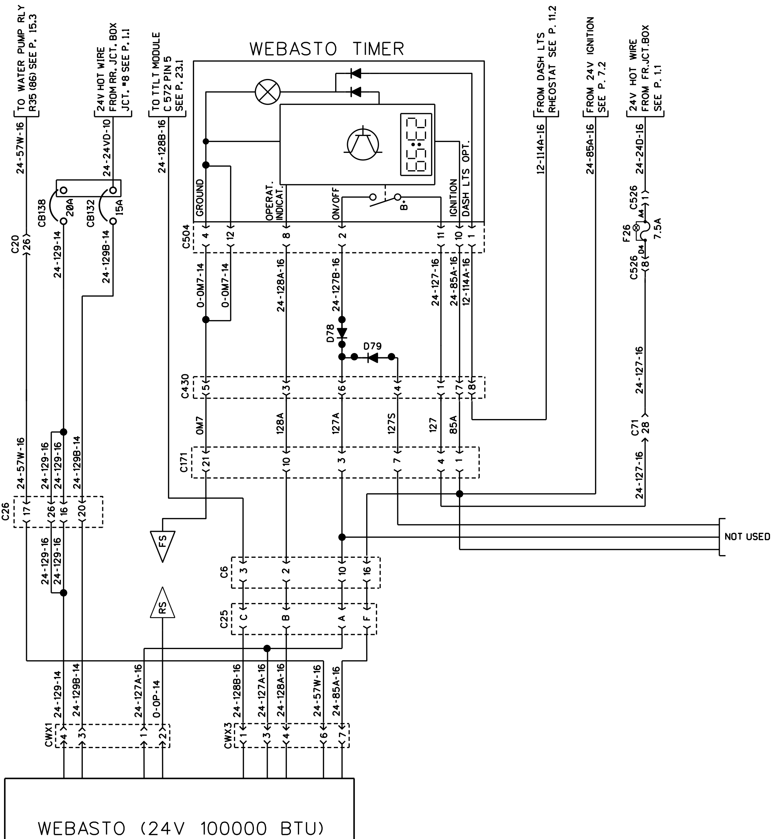
WEBASTO (24V 100000 BTU) PRE-HEAT WATER HEATER (WEBASTO THERMO 300)
