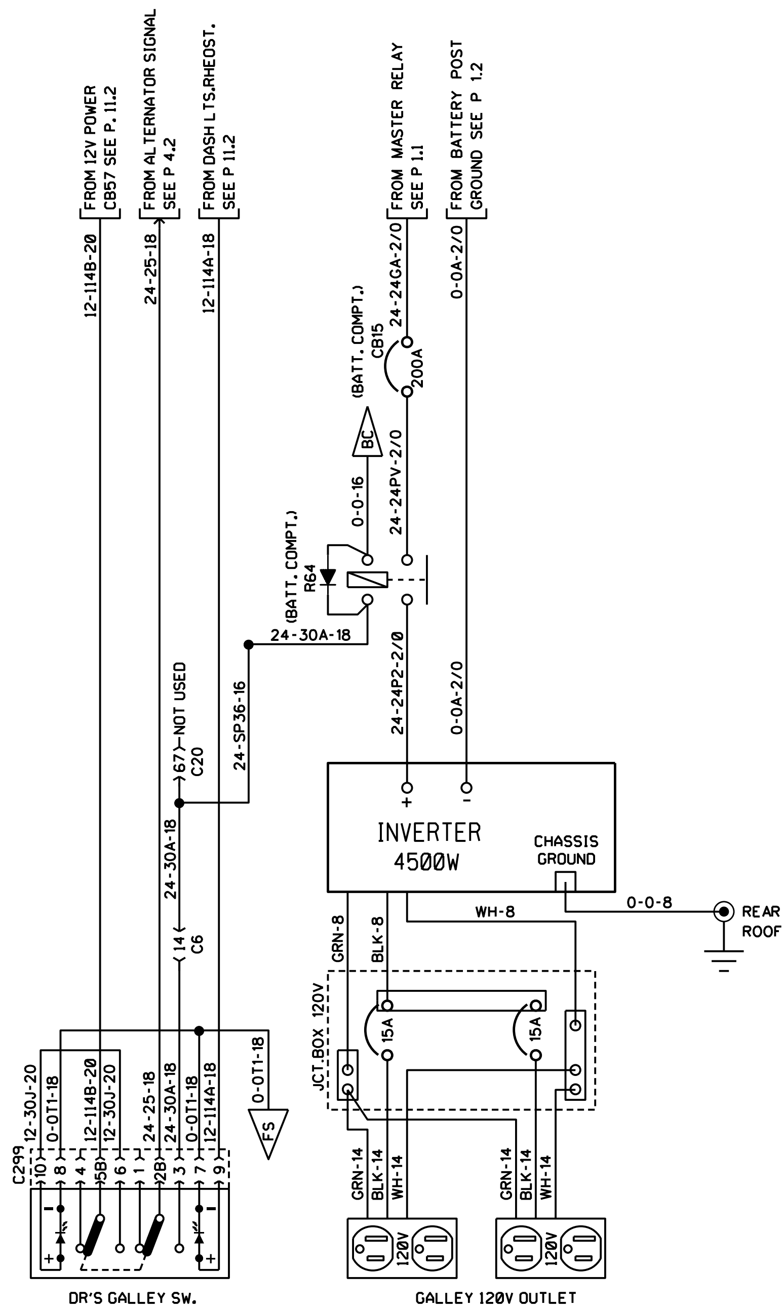
INVERTER GALLEY
