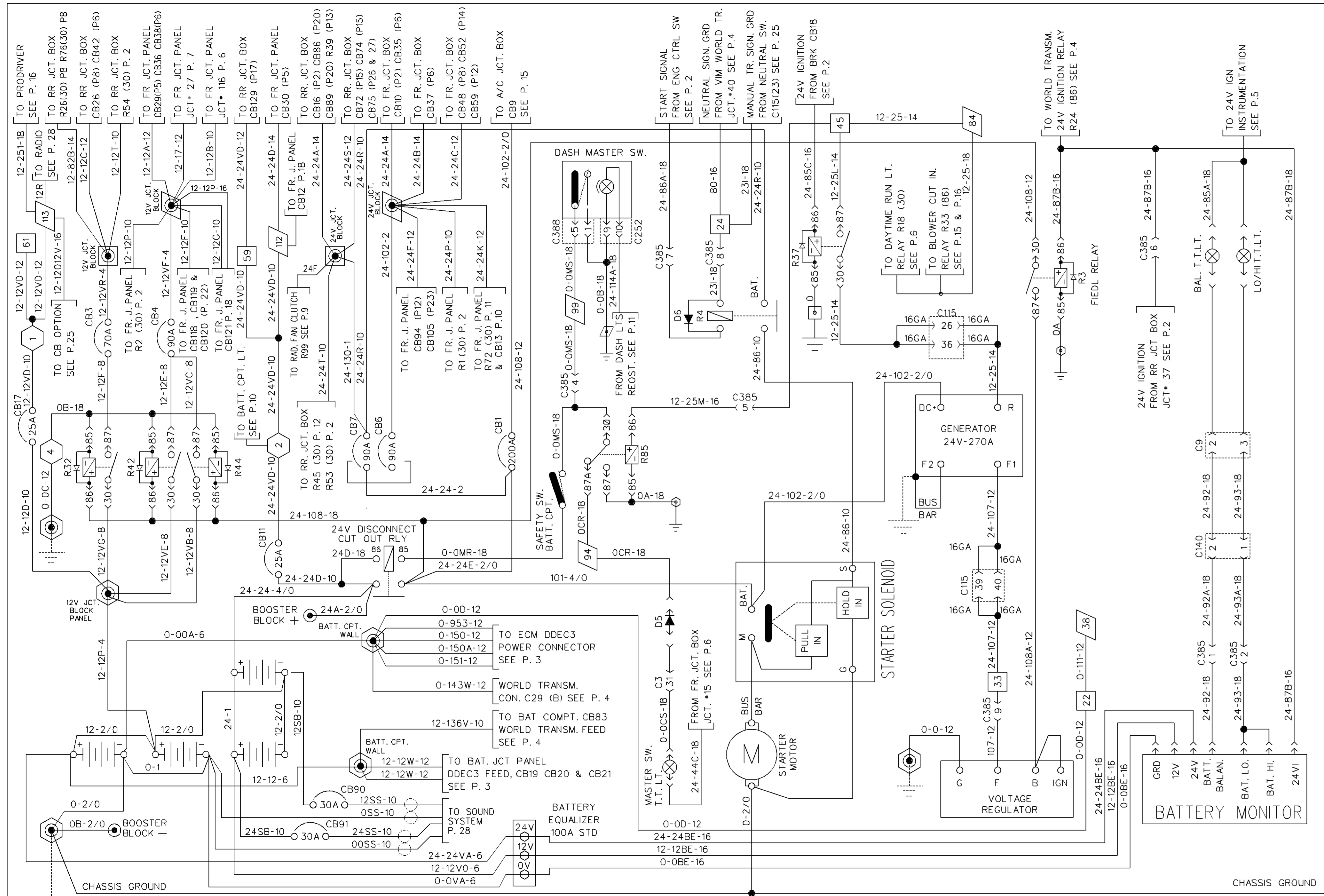
STD BATTERY CHARGING SYSTEM
