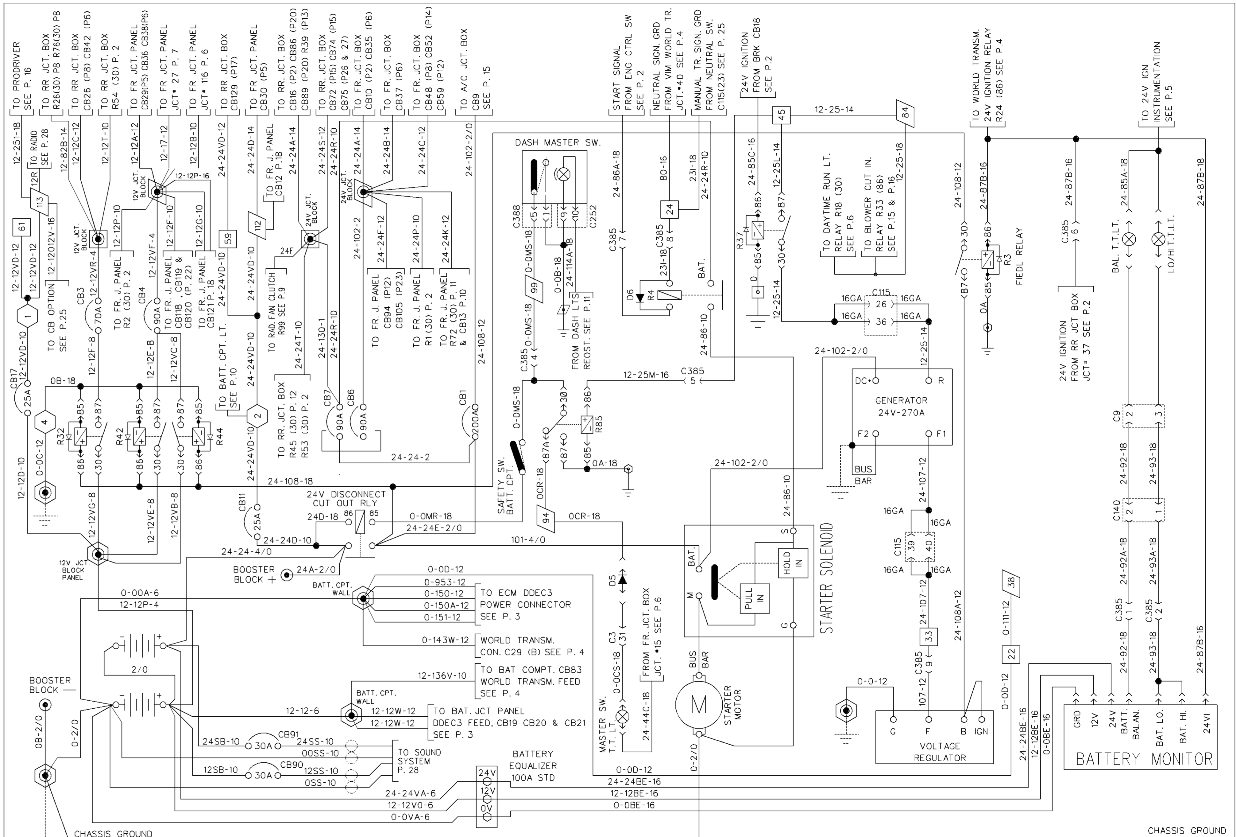
8D BATTERY CHARGING SYSTEM
