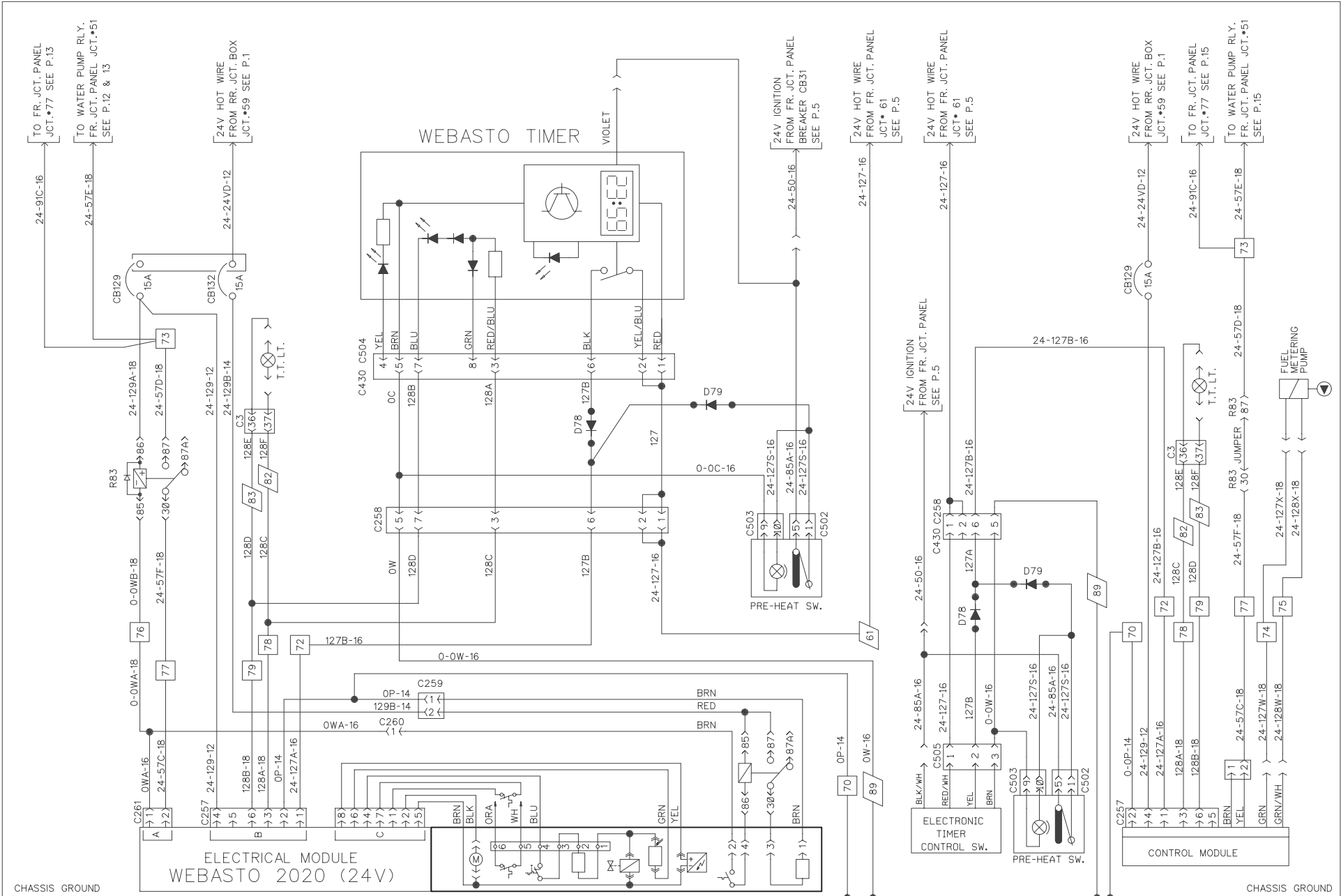
PRE-HEAT WATER HEATER WEBASTO 2020
