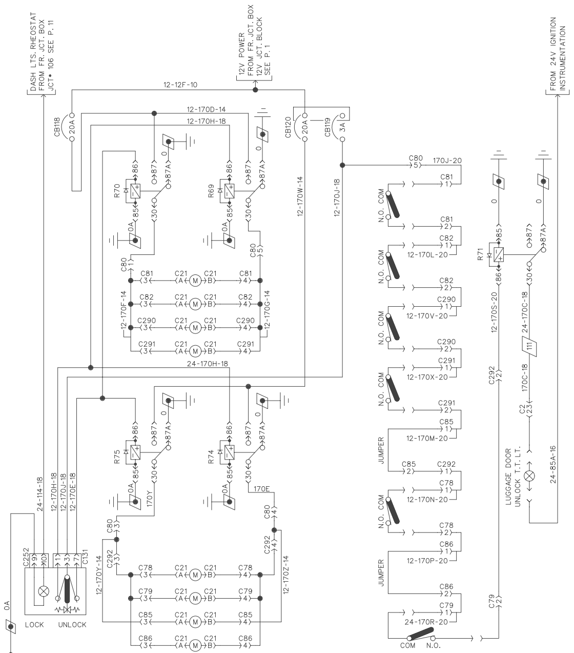
LUGGAGE DOOR LOCK.
