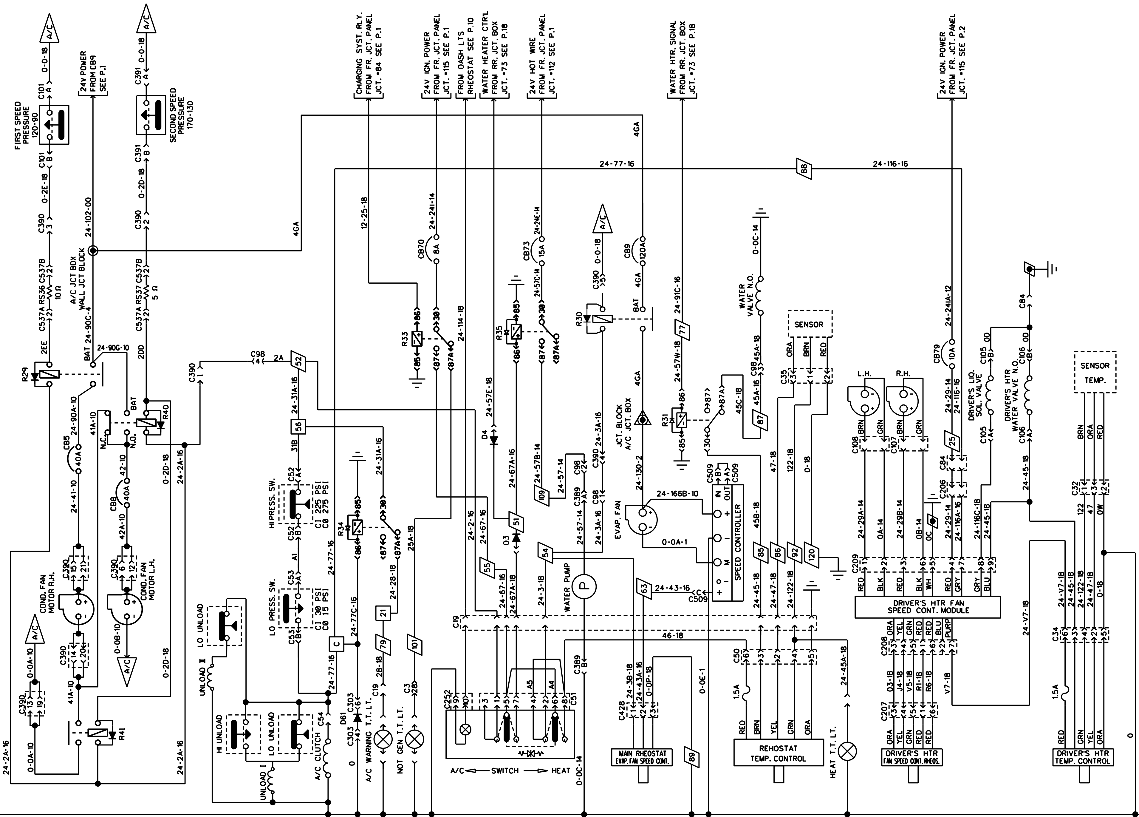
A/C AND HEAT SYSTEM (FULL AIR)
