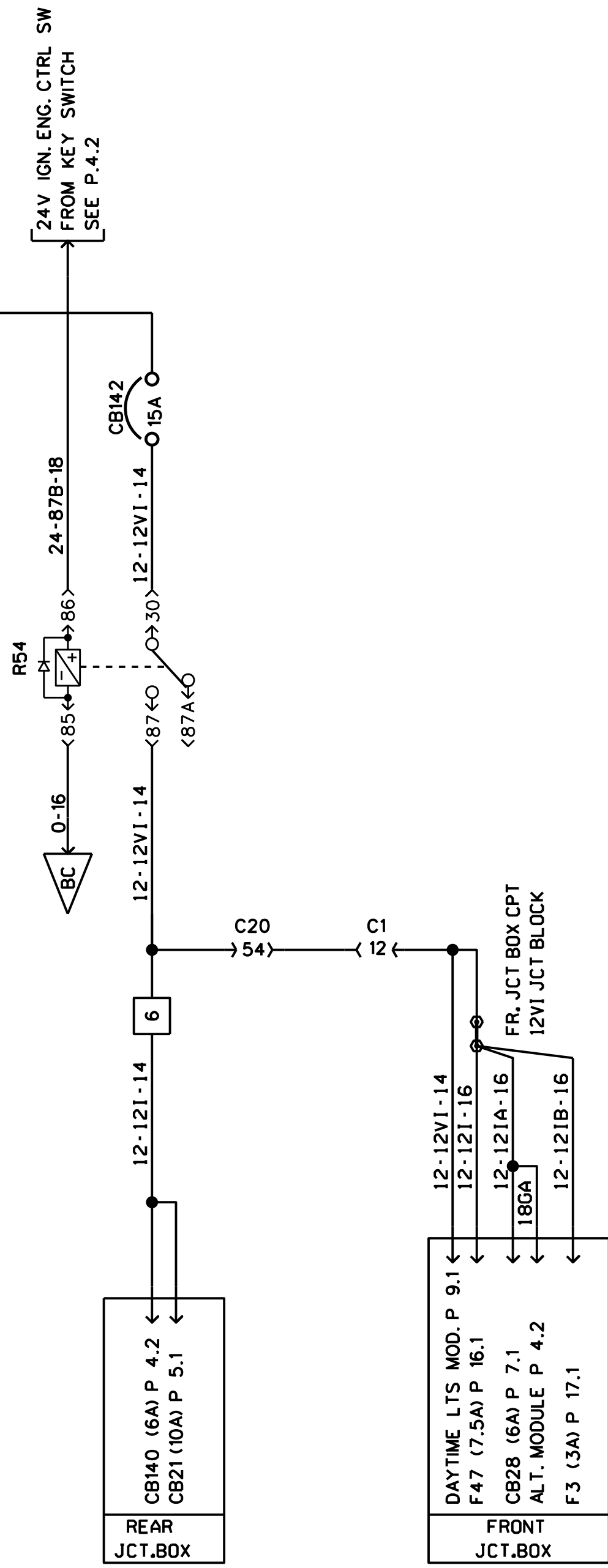
12V IGNITION
