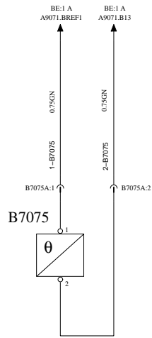
PASSENGER SENSOR, REHEATING SYS
