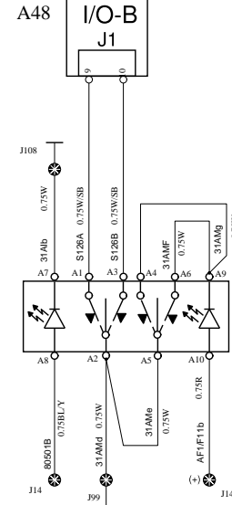
S126 SWITCH, DRIVER WINDOW
