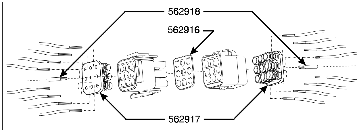
FIGURE 1: TYPICAL RAMCO MIRROR CONNECTOR SEAL INSTALLATION
