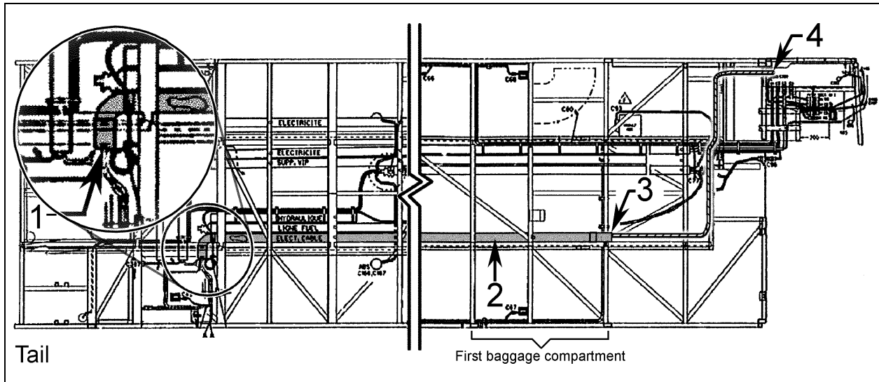
Figure 6: Top view of the structure. (1) Plastic elbow: entrance of the new #063365 cable; (2) Plastic tube, new cable's route; (3) End of the plastic tube; (4) End of the cable reaching the front service compartment.
