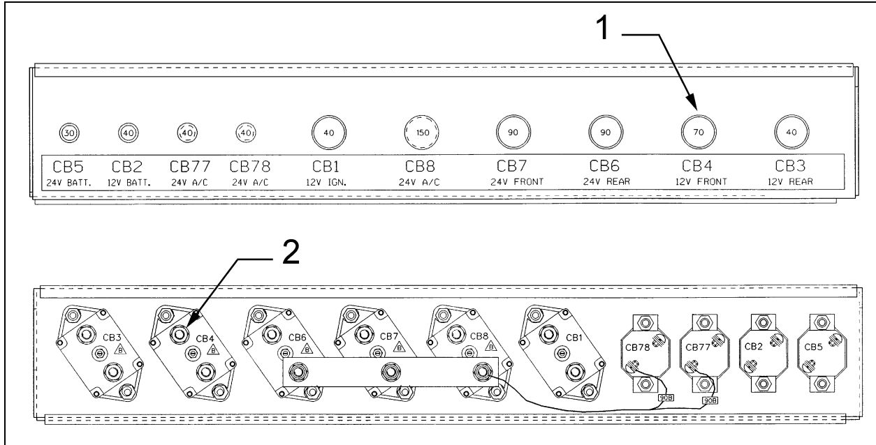
Figure 2: (1) Front view of the CB4 circuit breaker; (2) Rear view of the CB4 circuit breaker.
