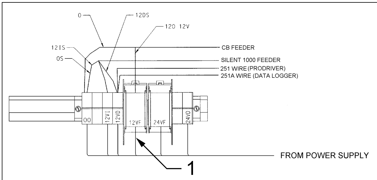
Figure 4: Front service compartment. (1) Cable to replace.
