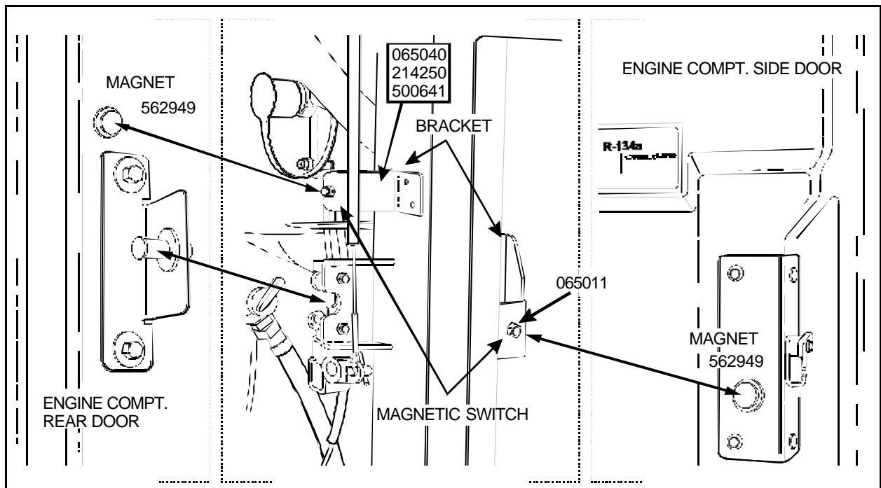
INSTALLATION OF MAGNETIC SWITCHES ON REAR AND RIGHT-HAND SIDE ENGINE DOORS
