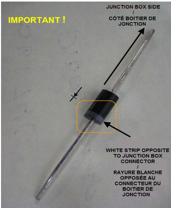
Fig.10 3amp diode installation.
