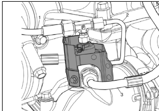
FORMER HARD FUEL LINE DESIGN
