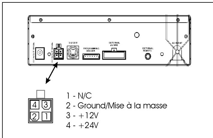
DVD PLAYER BACK PANEL
