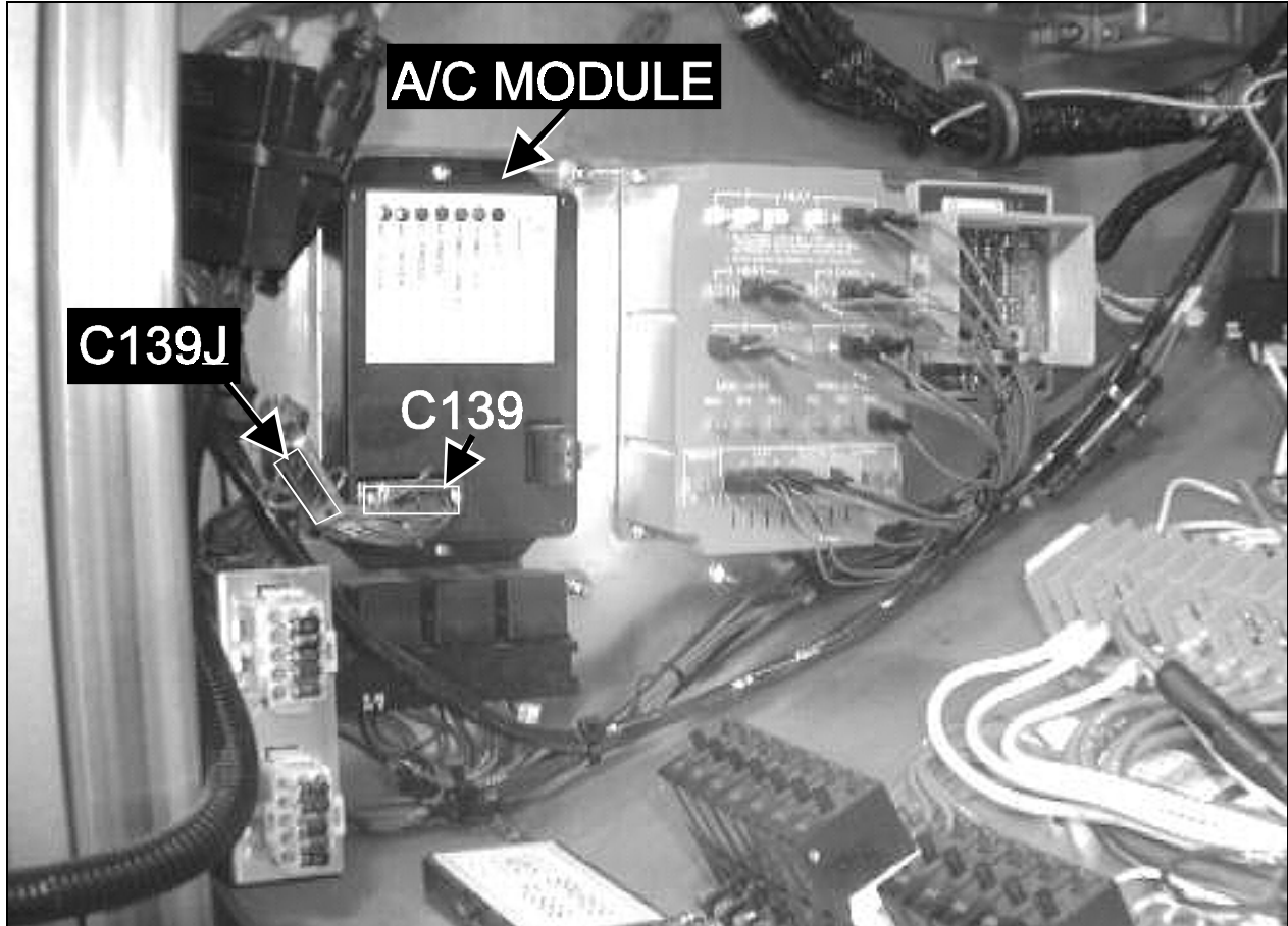
INSIDE OF L.H. REAR ELECTRIC COMPARTMENT
