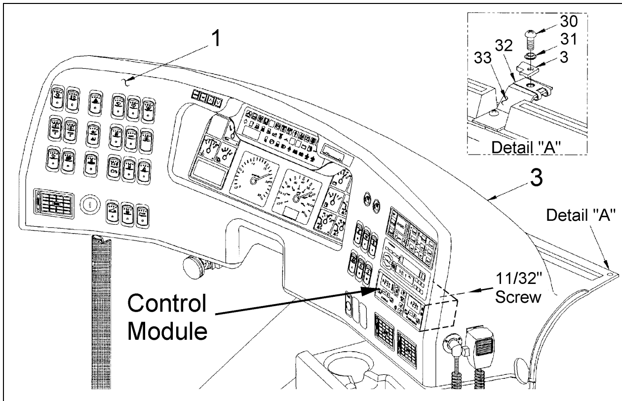
Figure 1: Control module of the HVAC. (1) Dashboard; (3) Dashboard cover panel; (30) M4 – 0,7 x 20 Screw (#5001411); (31) #500345 Washer; (32) #5001406 Spring nut; (33) Defroster installation part.
