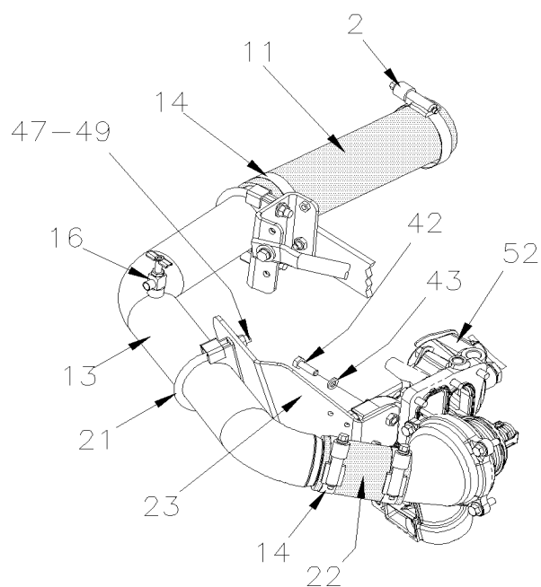
WITH "I-SHIFT" TRANSMISSION
