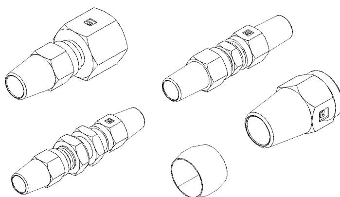
FITTING BRAKE "AB"
