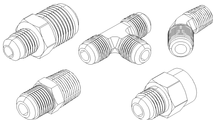
FITTING "SAE 45°"
