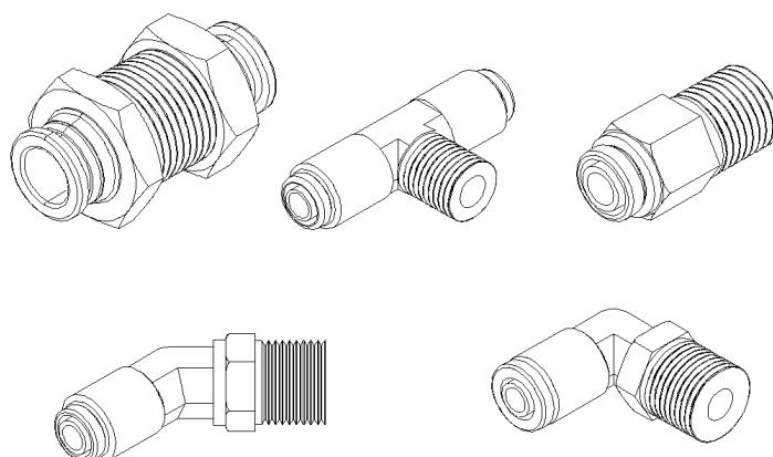
FITTING BRAKE "PUSH-IN"
