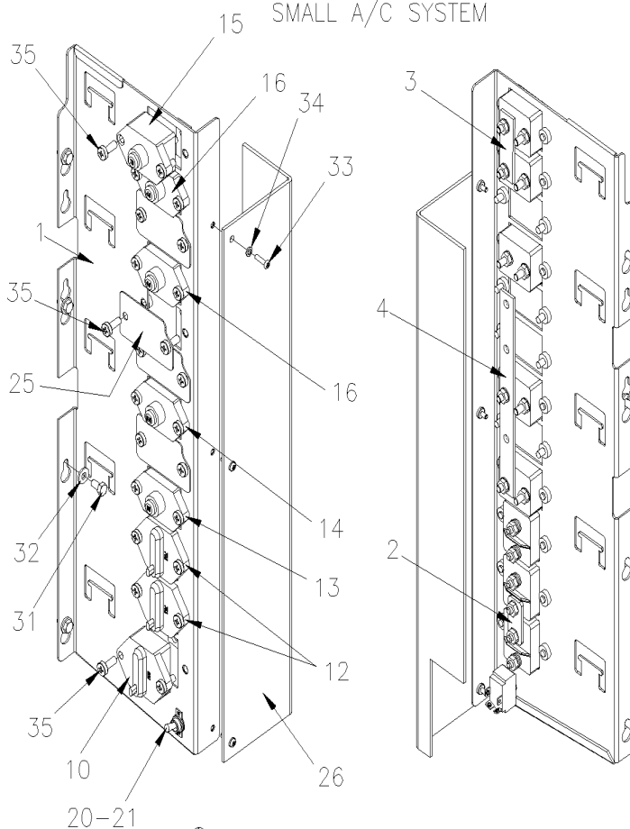
VIP WITH SMALL A/C SYSTEM
