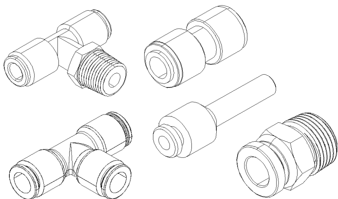
FITTING "PUSH-IN" 7
