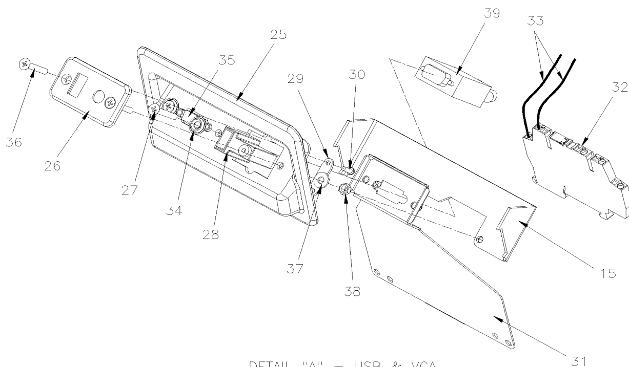
DETAIL "A" — USB &amp; VGA
