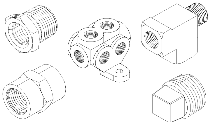
FITTING PIPE "NPT"
