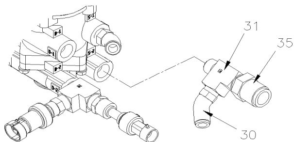
WITH TRAILER AIR BRAKE
