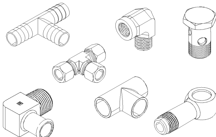
FITTING "MISCELANOUS" 12
