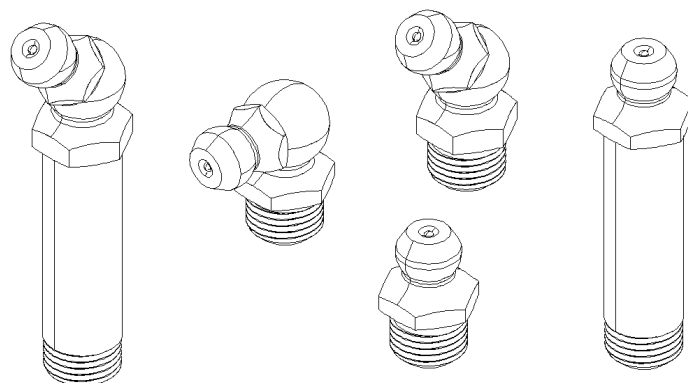
FITTING "GREASE" 30
