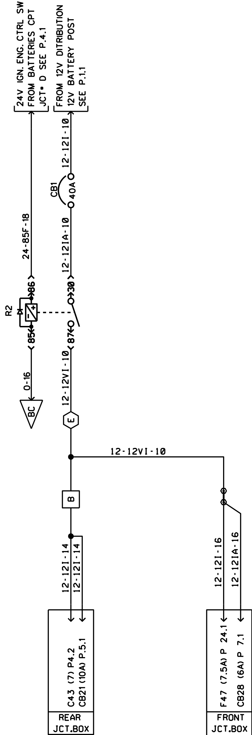
12V IGNITION
