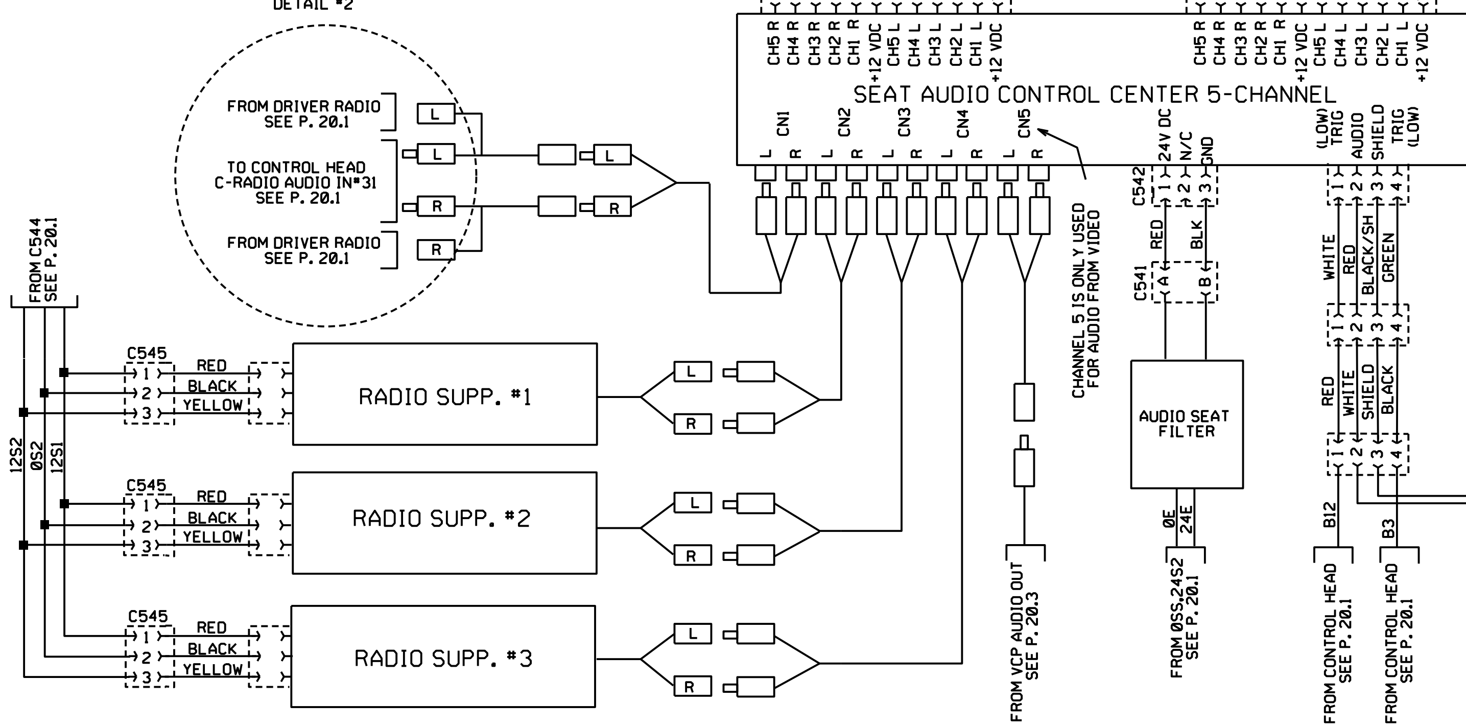
5-CHANNEL SLIM-LINE SEAT AUDIO SYSTEM
